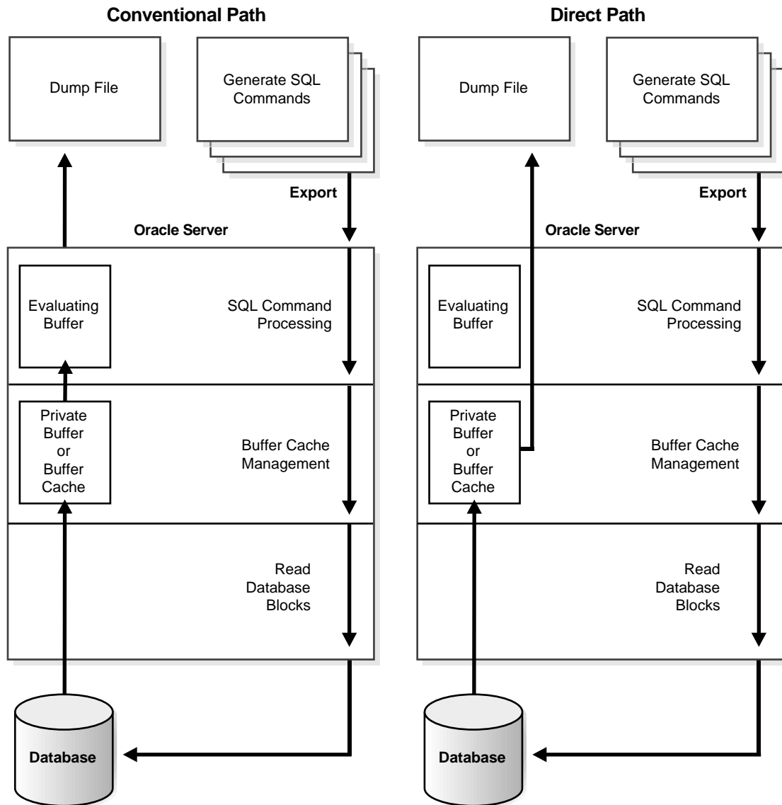
Figure 1-2 Database Reads on Conventional Path and Direct Path
