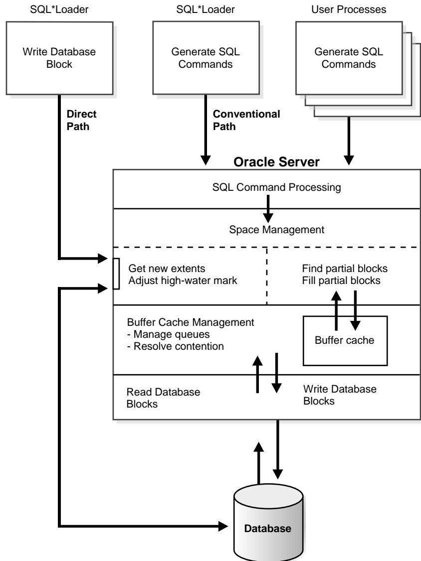
Figure 9–1 Database Writes on Direct Path and Conventional Path
