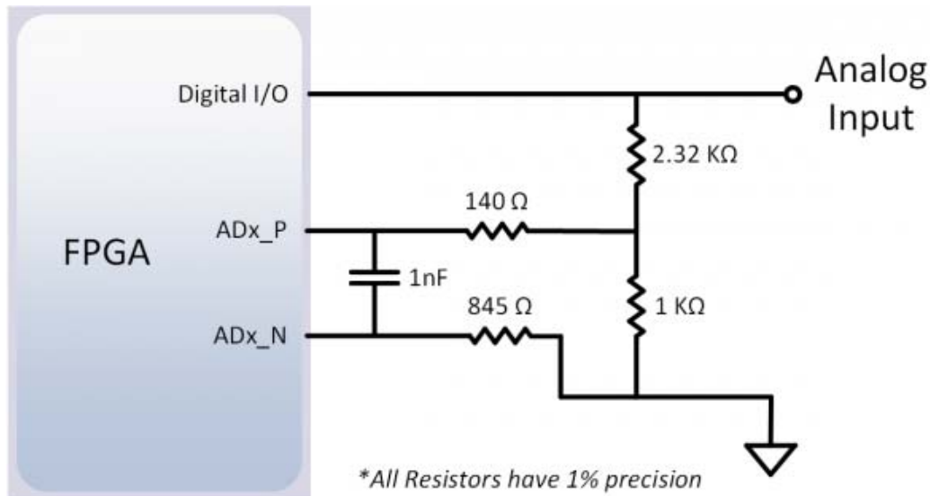
Figure 11.2.1 Arty A7 Single-Ended Analog Inputs
