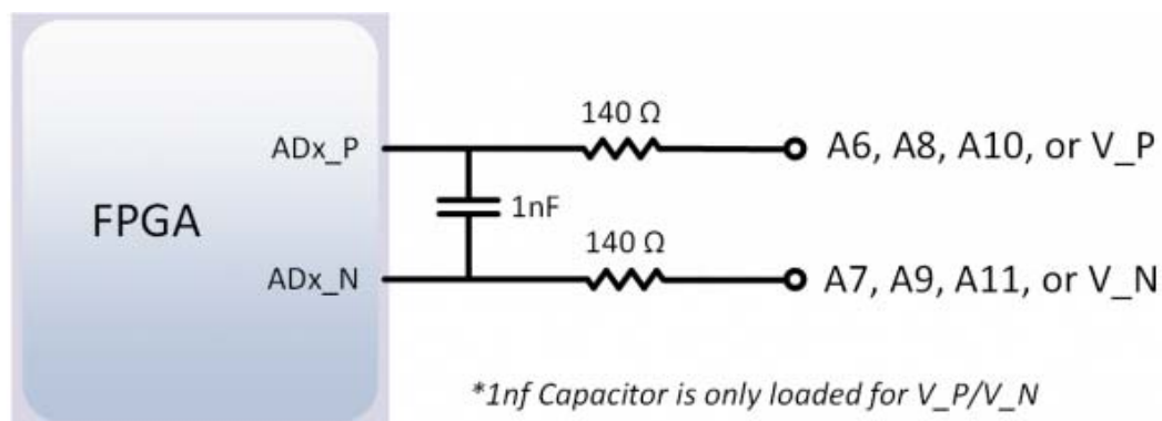
Figure 11.2.2 Arty A7 Differential Analog Inputs
