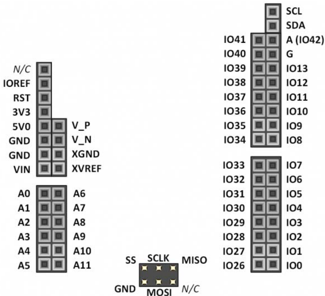
Figure 11.1 diagrams the pins found on the shield connector of the Arty A7.
