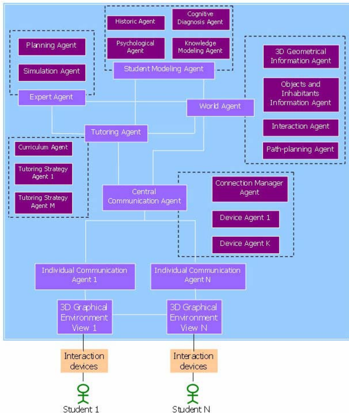
Fig. 2 Agent-based architecture
