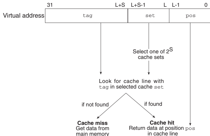
Figure 5-1 Cache look-up
