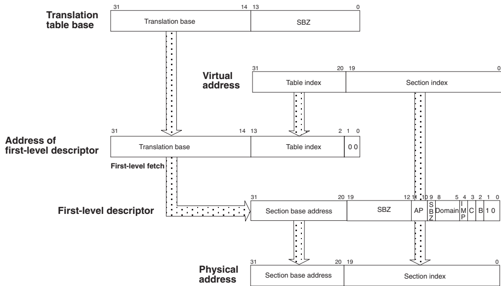
Figure 3-3 Section translation
