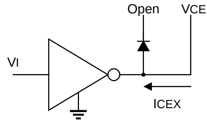
Figure 2 ICEX Test Circuit
