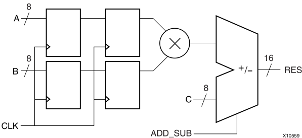
Multiplier Adder With 2 Register Levels on Multiplier Inputs Diagram
