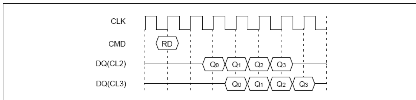
Figure 6-6. CL (CAS Latency) Timing Diagram
