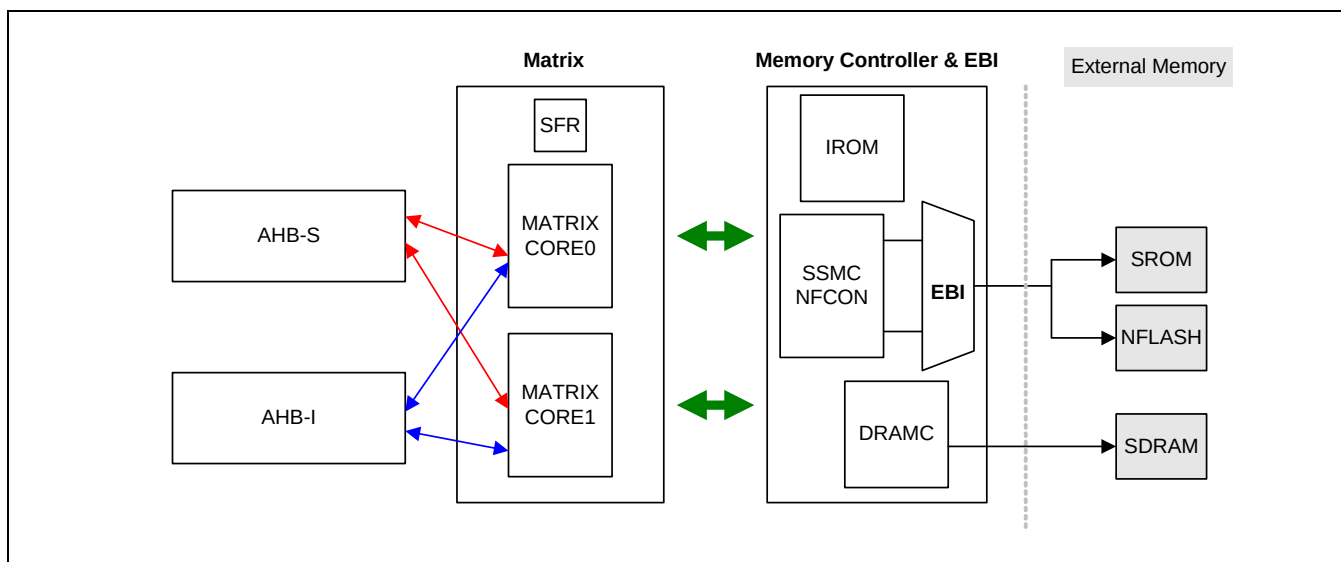
Figure 3-1. The Configuration of MATRIX and Memory Sub-System of S3C2416
