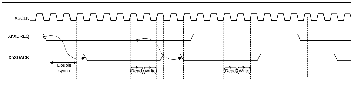
Figure 8-4. Single service, Demand Mode, Single Transfer Size
