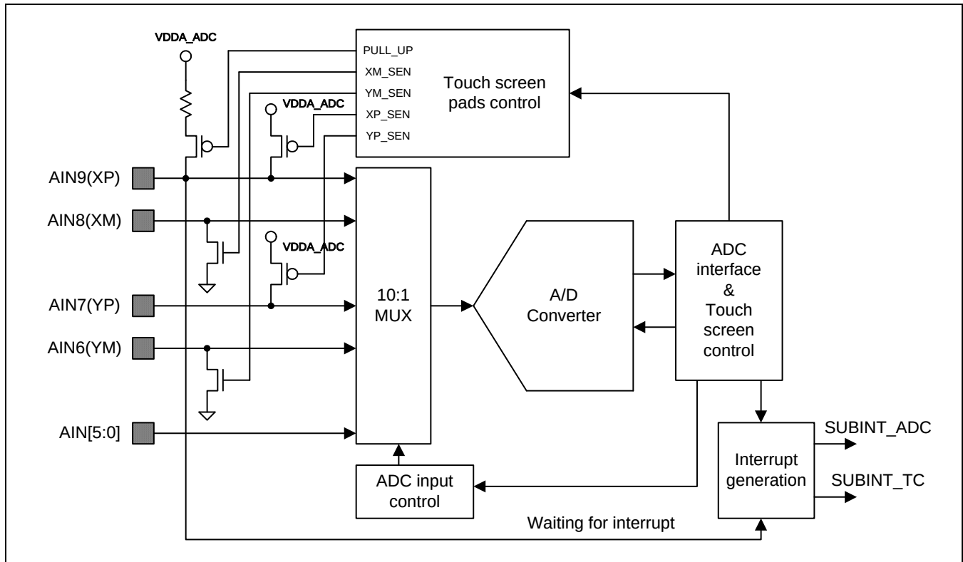
Figure 22-1. ADC and Touch Screen Interface Block Diagram
