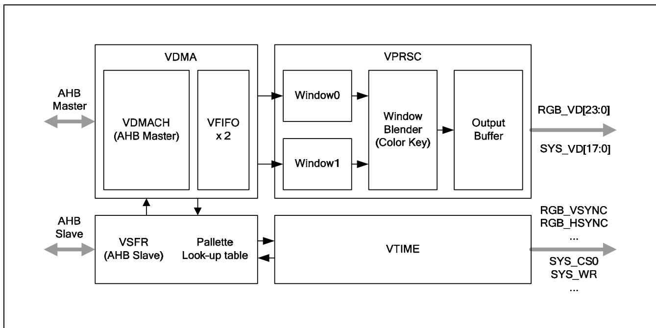
Figure 21-1. LCD Controller Block diagram
