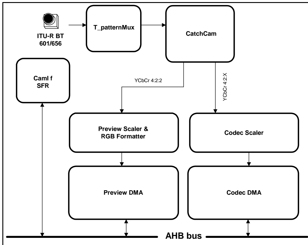
Figure 23-1 CAMIF Overview
