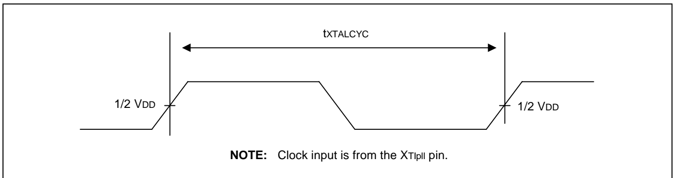
Figure 27-2 XT1P11 Clock Timing Diagram
