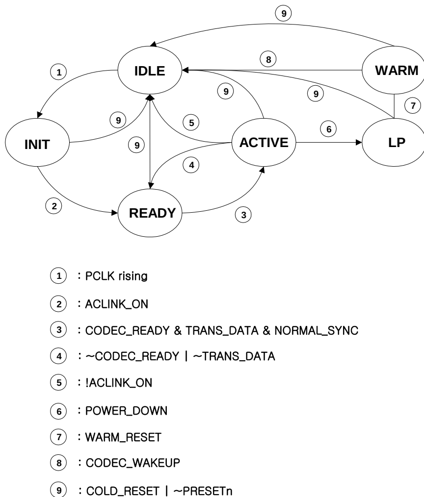
Figure 35-8. AC97 State Diagram
