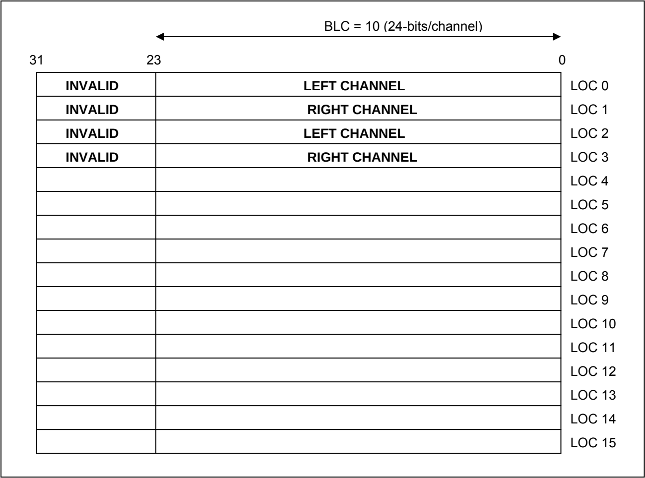
Figure 36-7. RX FIFO Structure for BLC = 10 (24-bits/channel)
