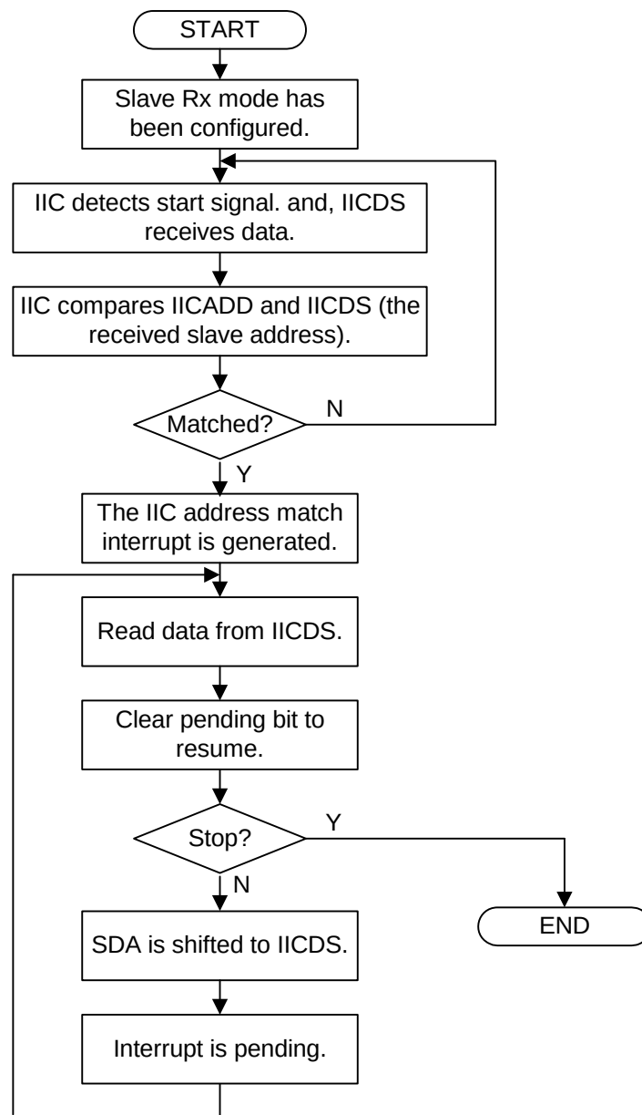
Figure 30-9. Operations for Slave/Receiver Mode
