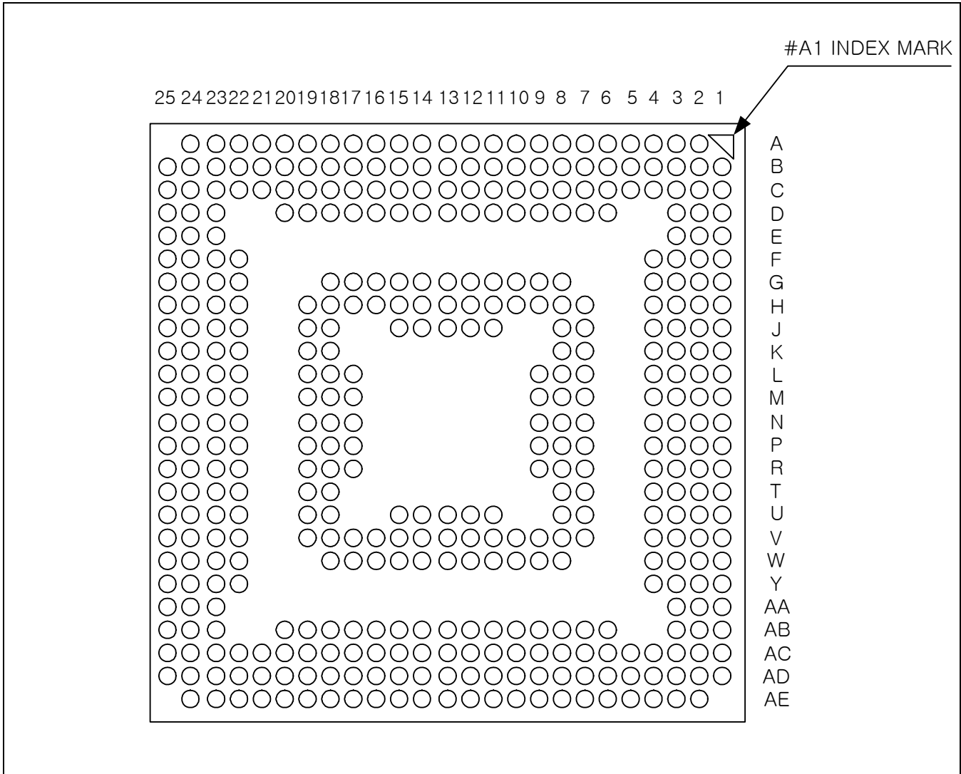
Figure 1-2. Pin Assignments
