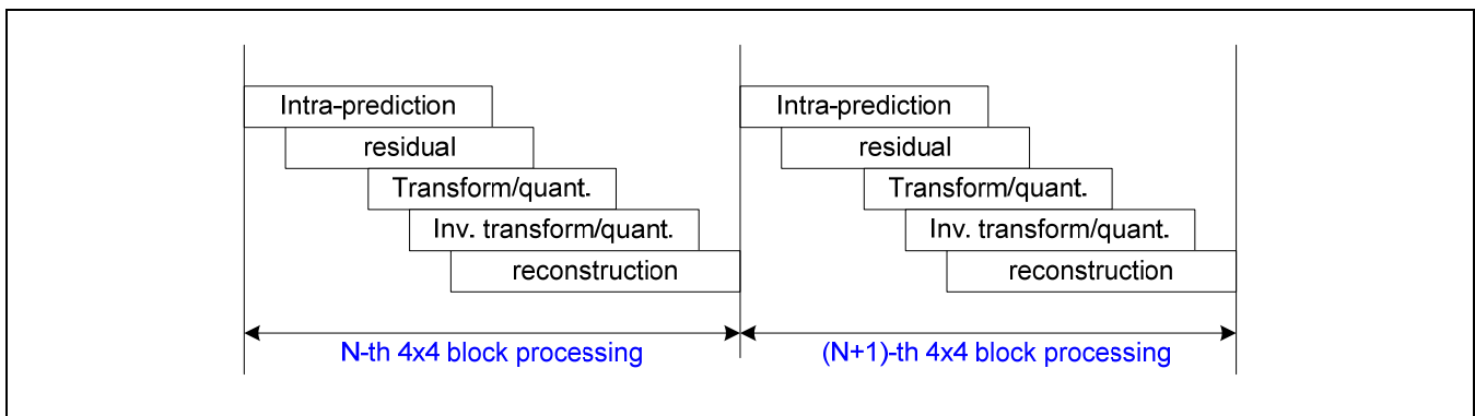
Figure 21-22 H.264 encoding pipeline
