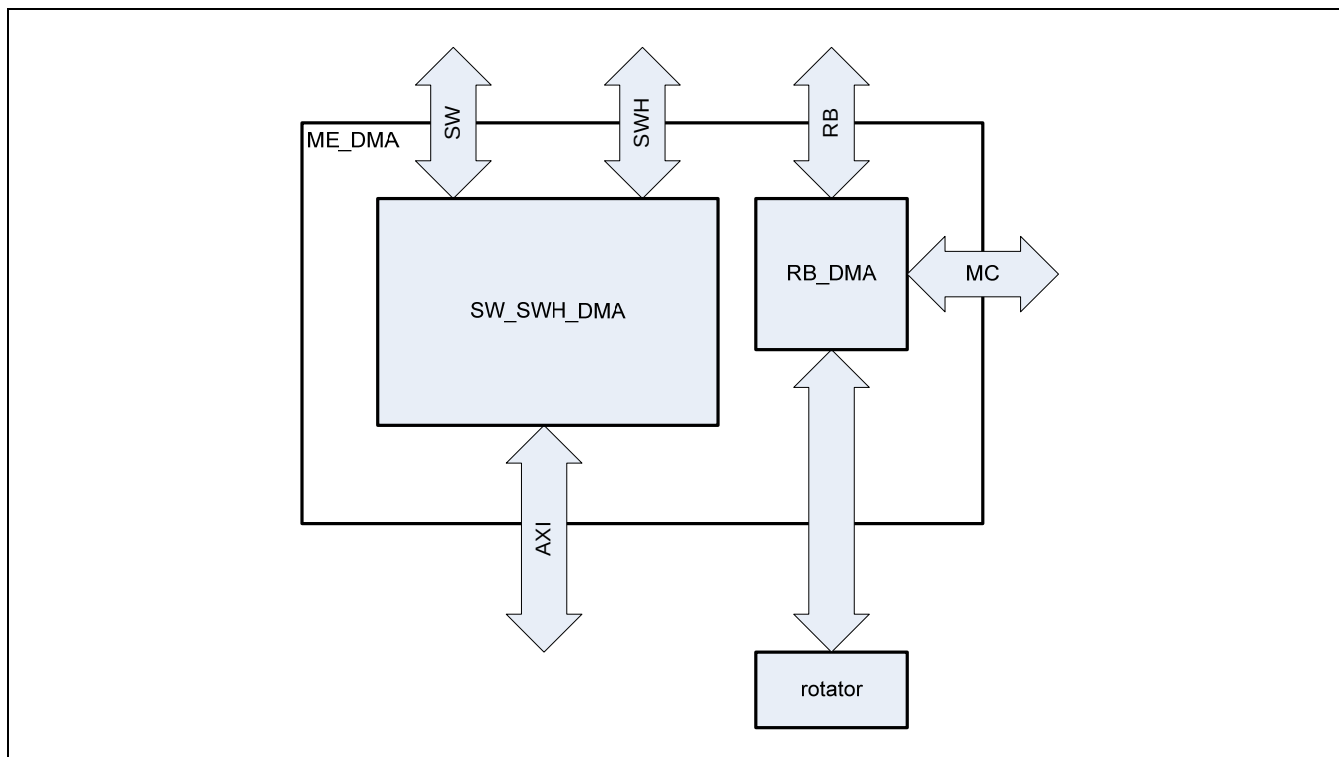
Figure 21-15. Motion Estimation DMA Block Diagram
