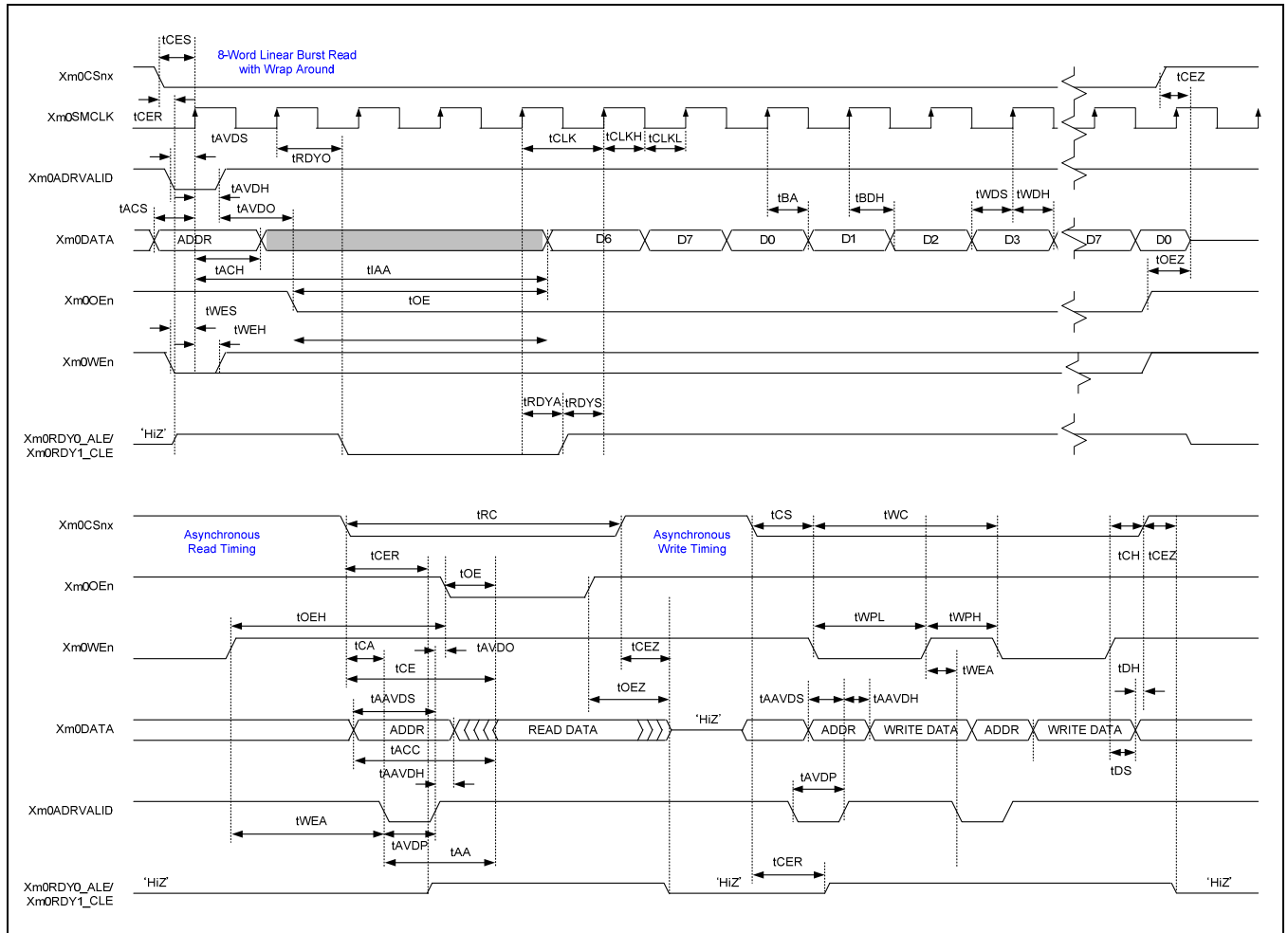
Figure 44-8. OneNand Flash Timing
