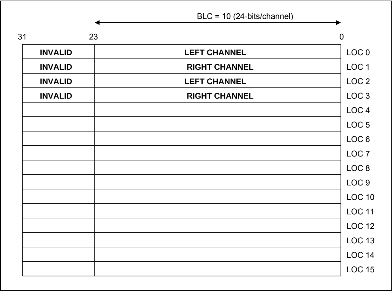
Figure 36-5. TX FIFO Structure for BLC = 10 (24-bits/channel)
