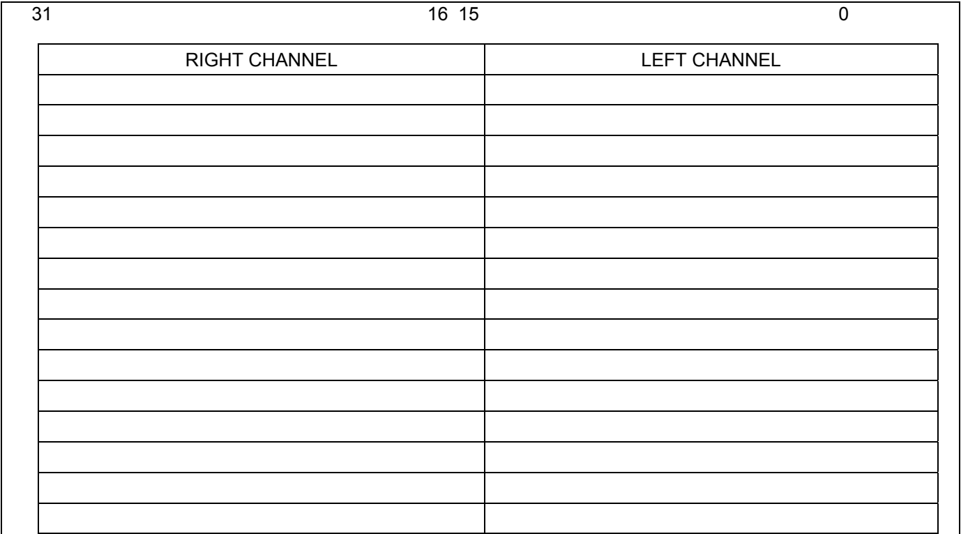
Figure 36-4. TX FIFO Structure for BLC = 00 or BLC = 01
