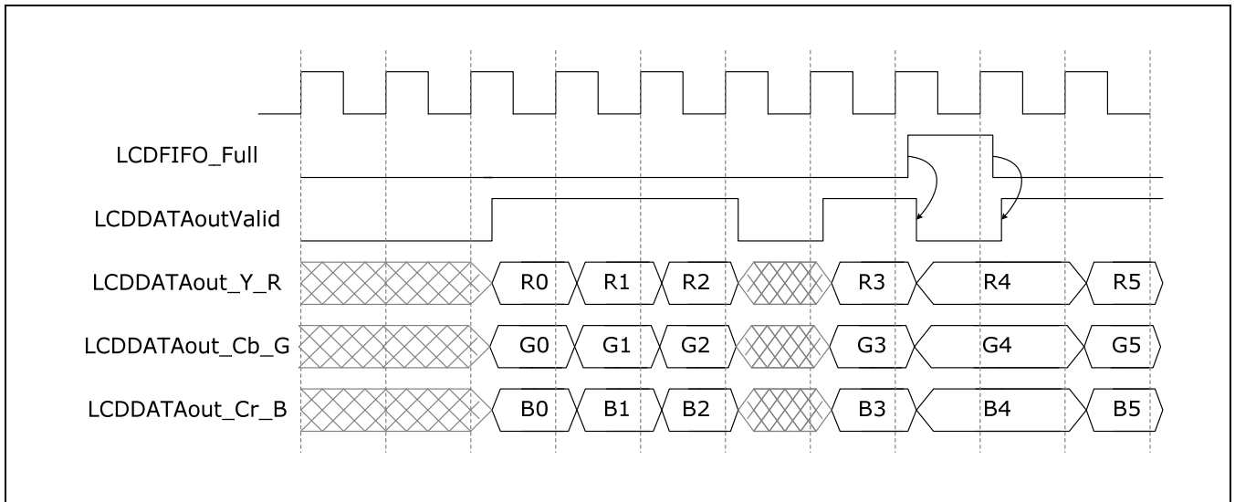
Figure 20-24. I/O Timing Diagram for LCD Path
