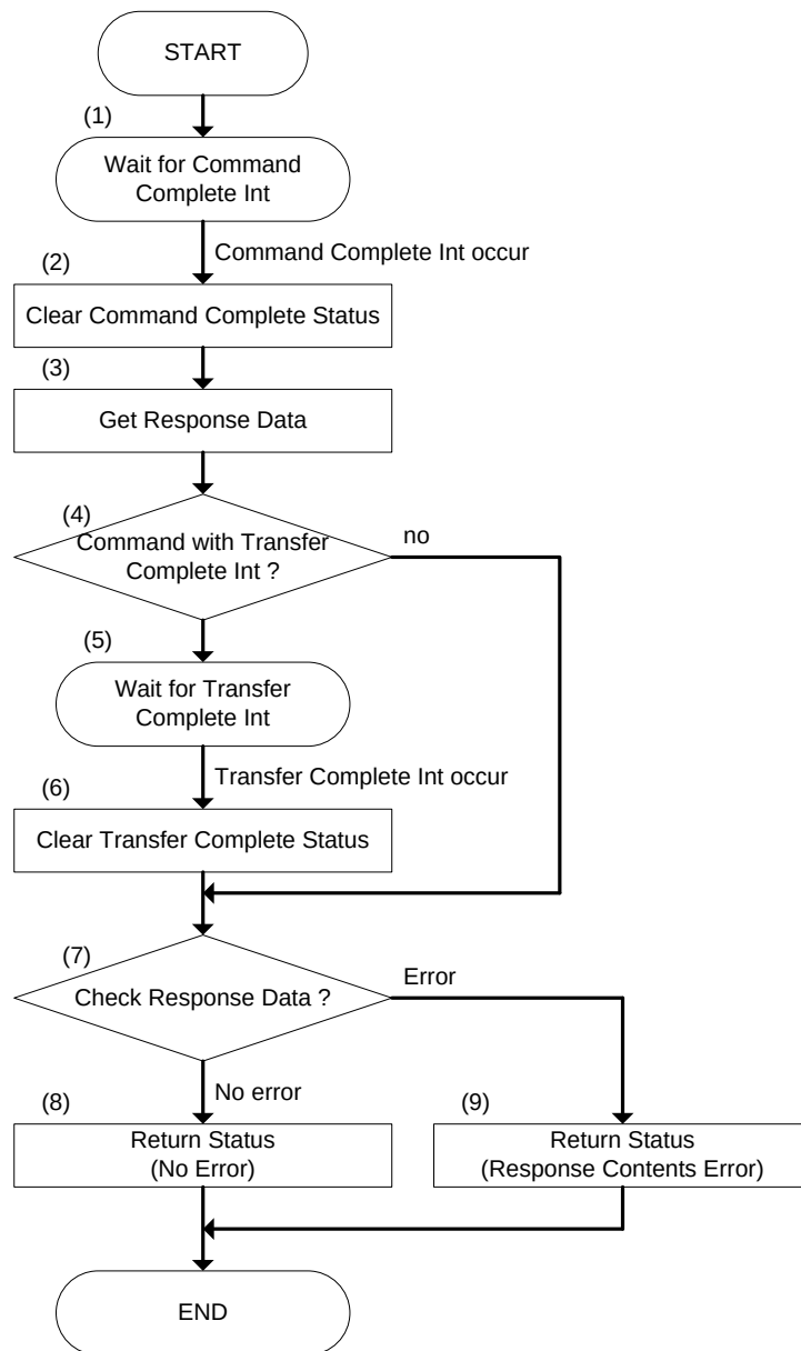
Figure 27-10. Command Complete Sequence
