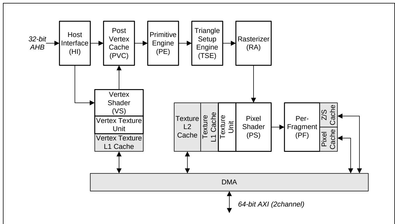
Figure 42-1. Block Diagram
