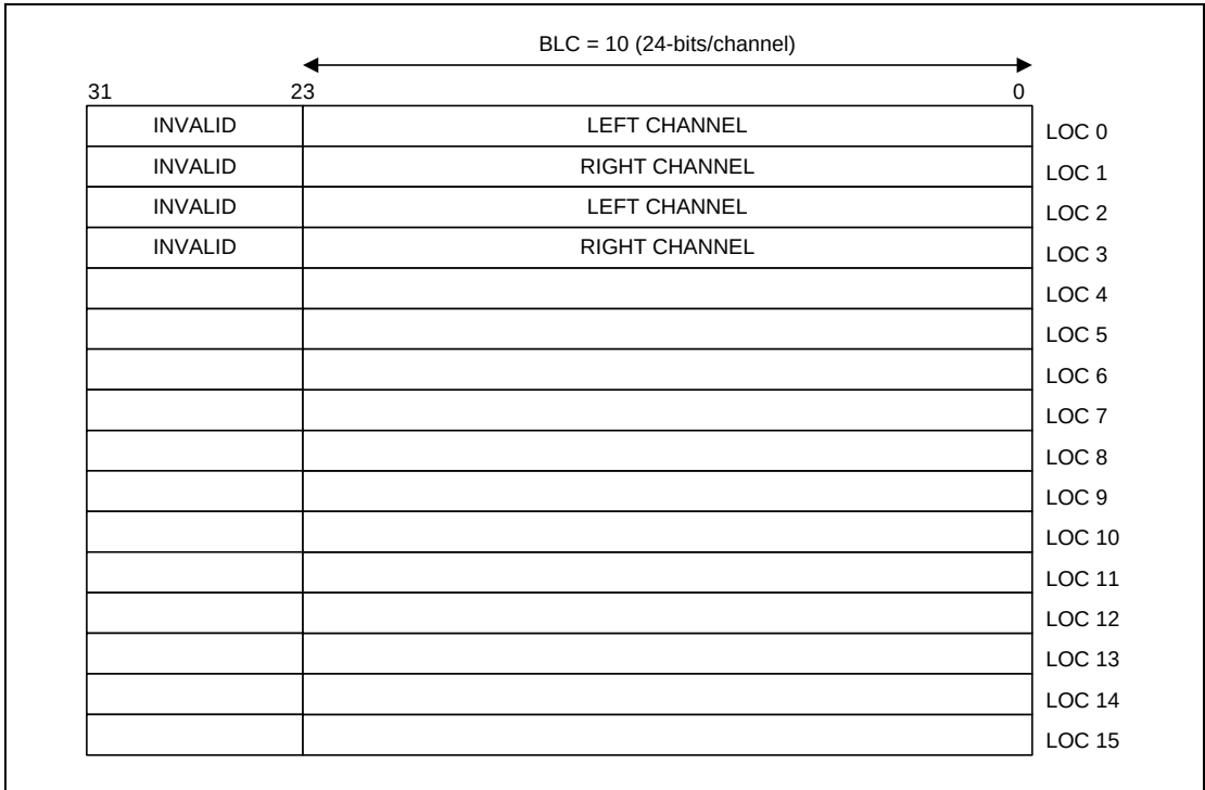
Figure 41-5. TX FIFO Structure for BLC = 10 (24-bits/channel)
