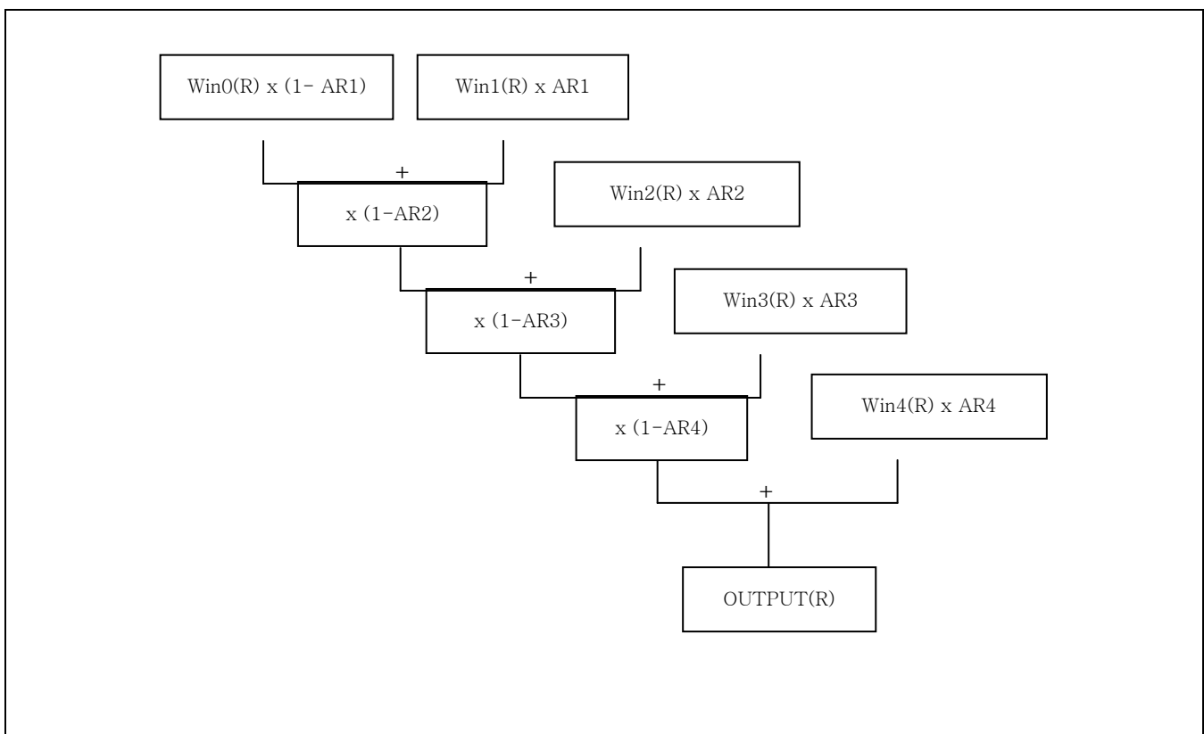
Figure 14-5. Blending diagram
