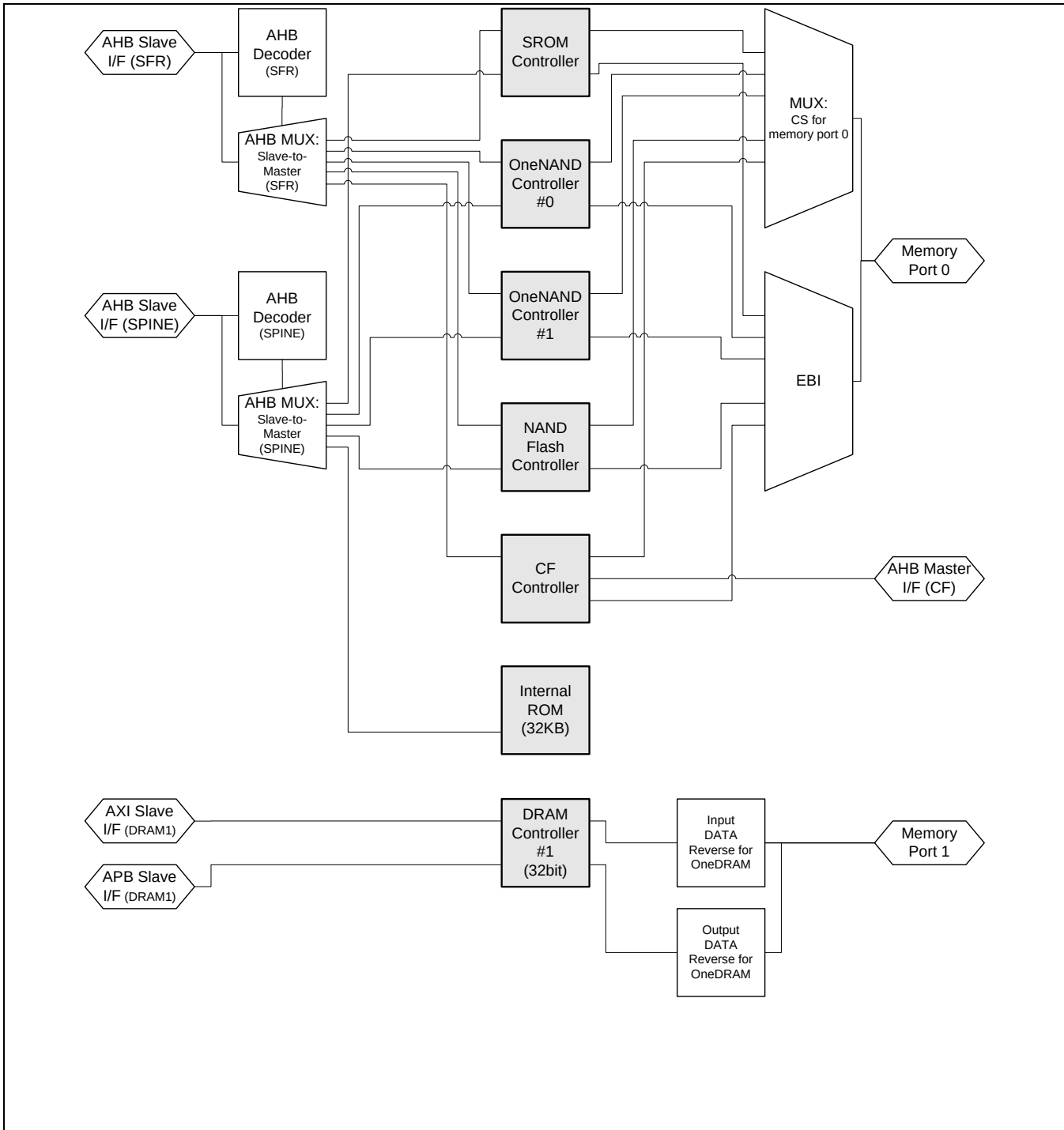
Figure 4-1 Structure of Memory Sub-system
