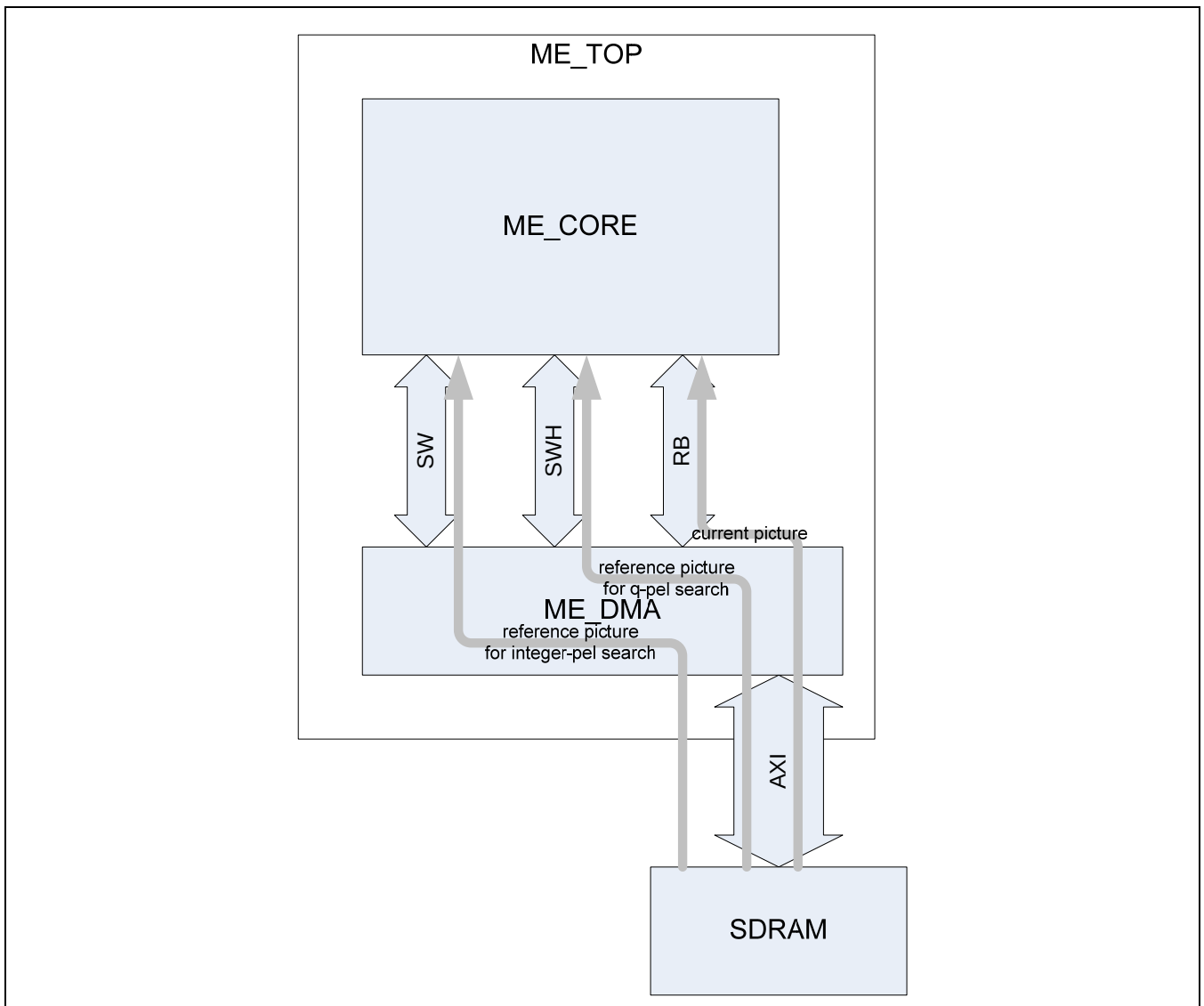
Figure 21-13. Motion Estimation Block Diagram
