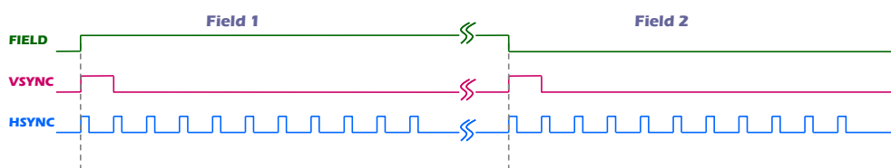
Figure 14-13. ITU-R BT.601 Controllable Vsync
