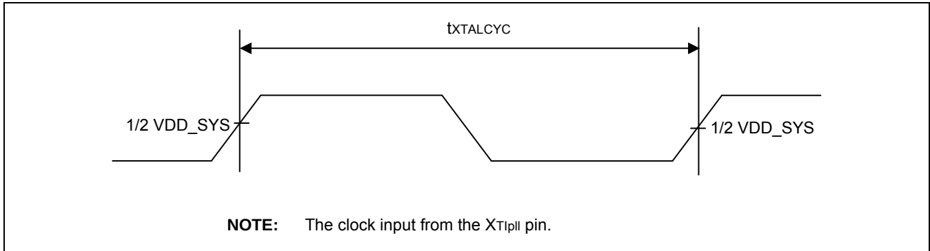
Figure 44-1. XT1p11 Clock Timing
