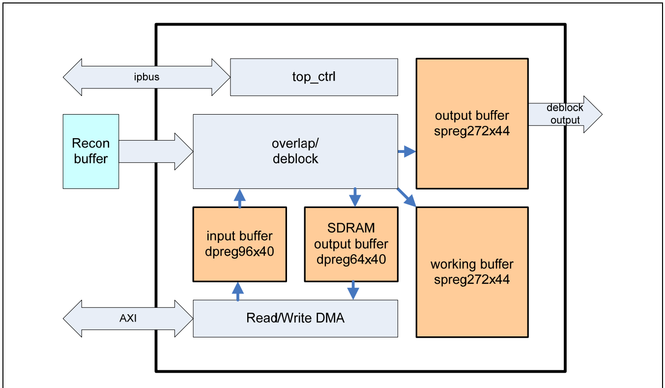
Figure 21-25. Overlap/deblocking filter architecture
