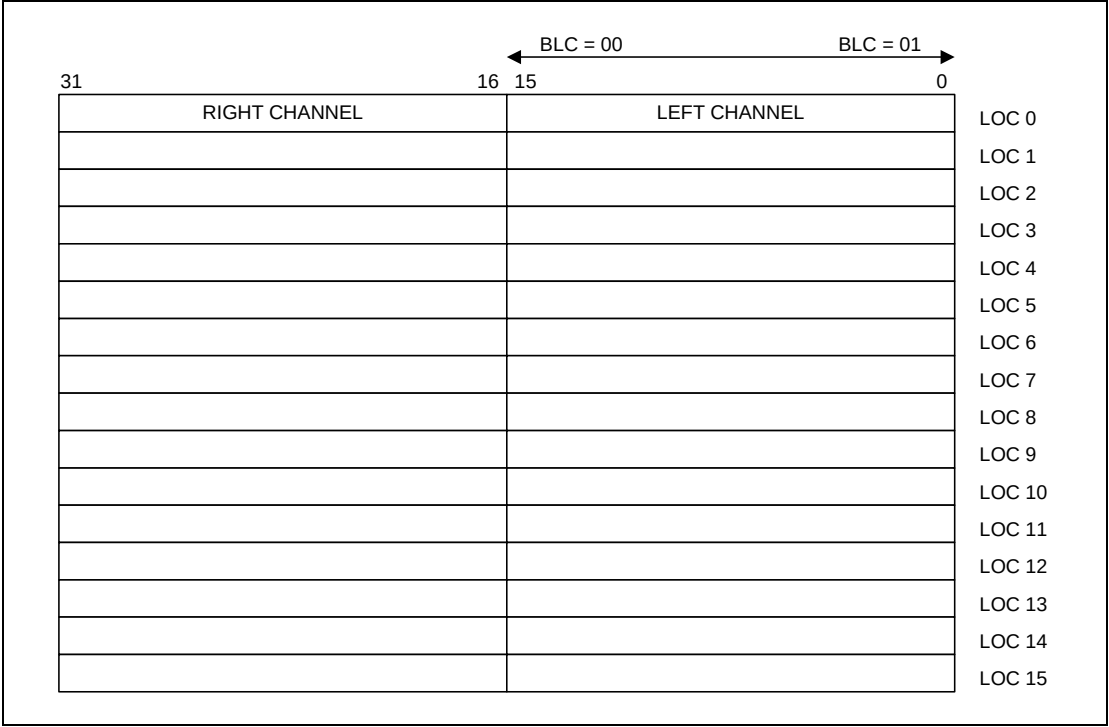
Figure 41-6. RX FIFO Structure for BLC = 00 or BLC = 01
