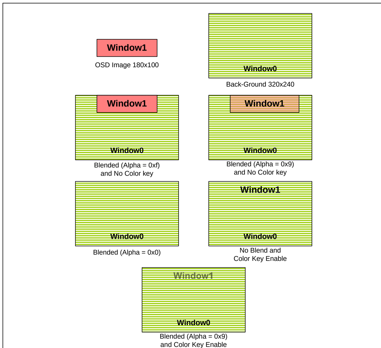
Figure 14-8. Color Key Function Configurations
