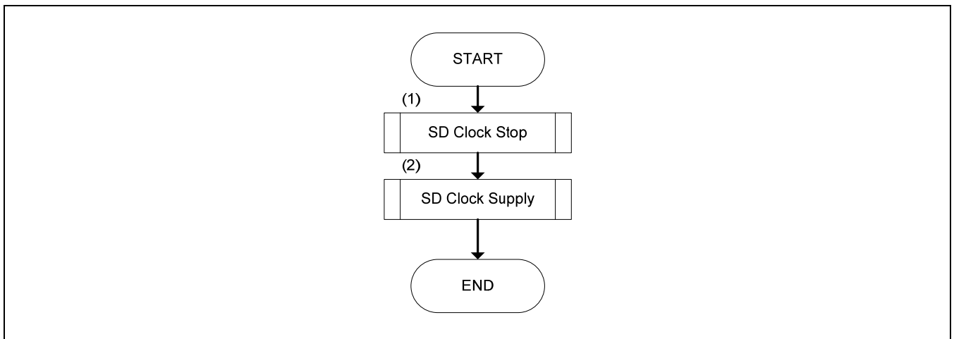
Figure 27-5. SD Clock Change Sequence
