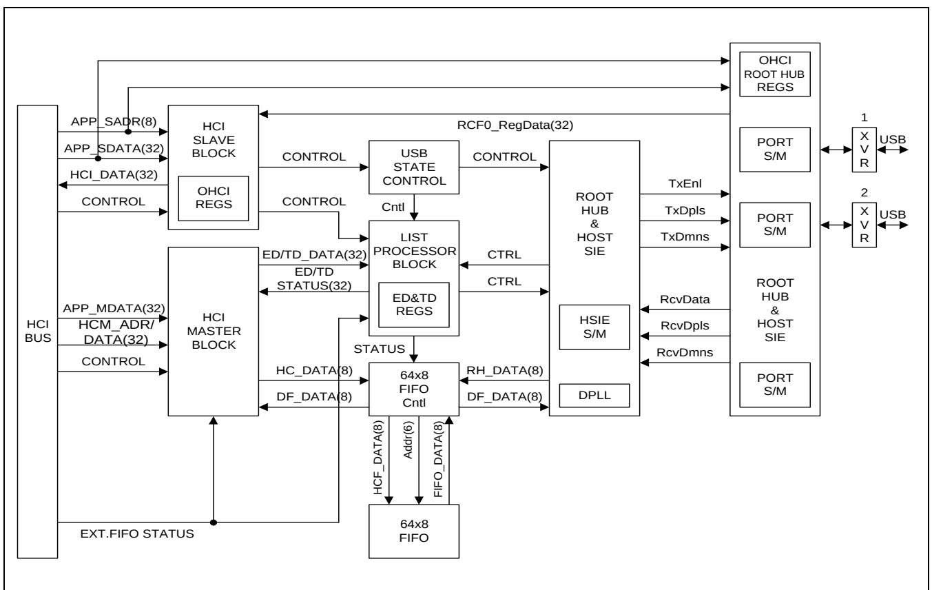
Figure 25-1. USB Host Controller Block Diagram
