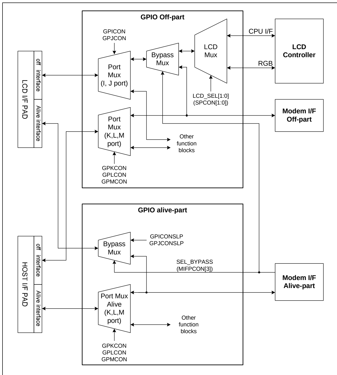
Figure 10-3. Diagram of LCD bypass logic
