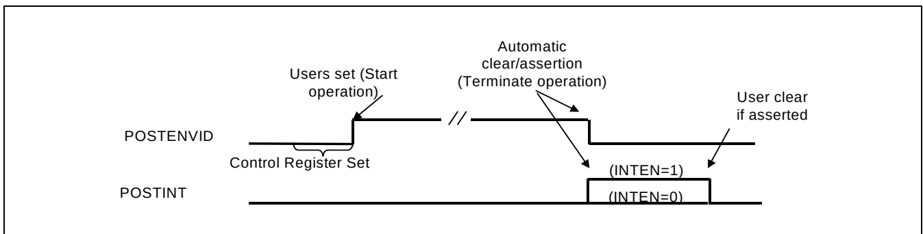
Figure 15-8. Start and termination of POST PROCESSOR operation (AutoLoadEnable = 0) Block Diagram
