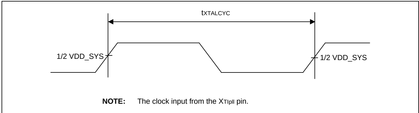
Figure 12.1- 1 XTlpII Clock Timing
