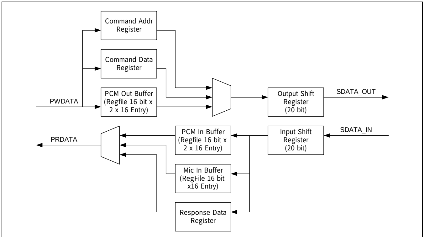
Figure 10.4-2 Internal Data Path
