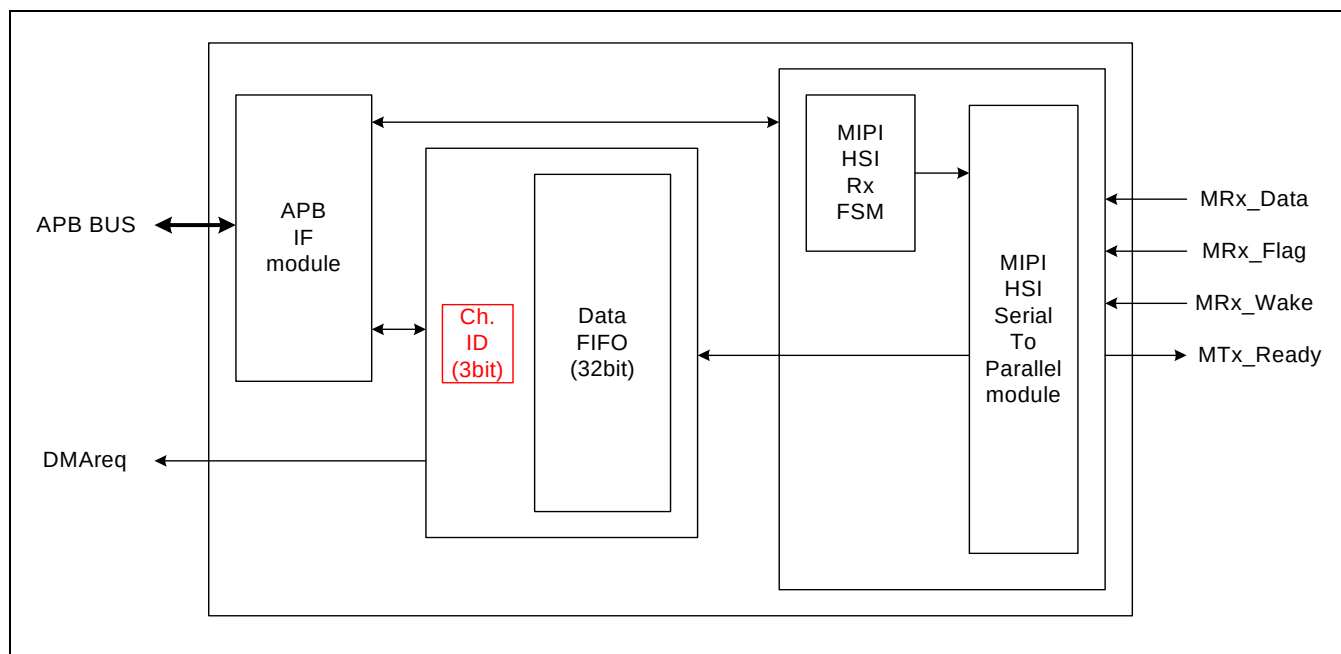
Figure 8.6-4 MIPI HSI Interface Controller Rx Module Top Block Diagram
