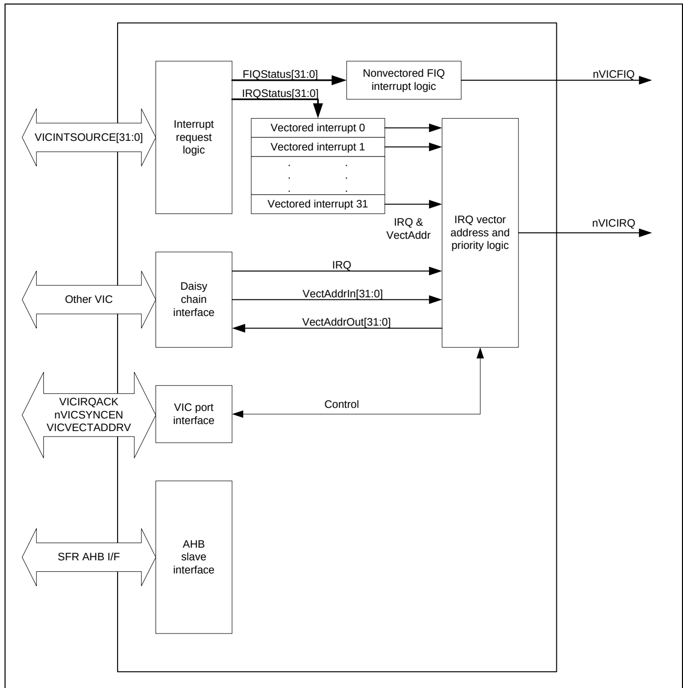
Figure 4.1-1 VICn Diagram
