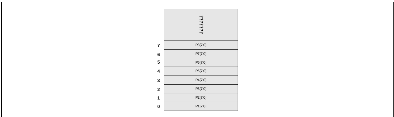
Figure 8.8-4 RAW8 Data Storing Order
