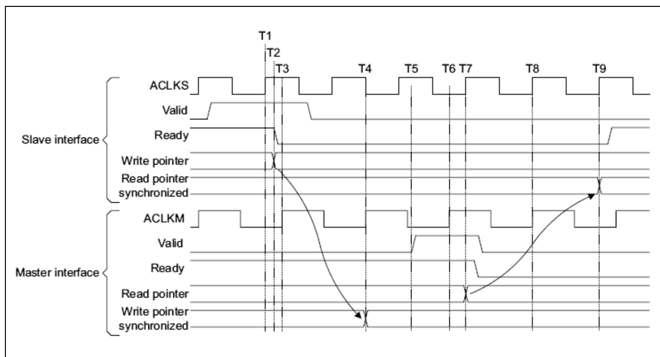
Figure 3.4-4 Single Place FIFO Timing
