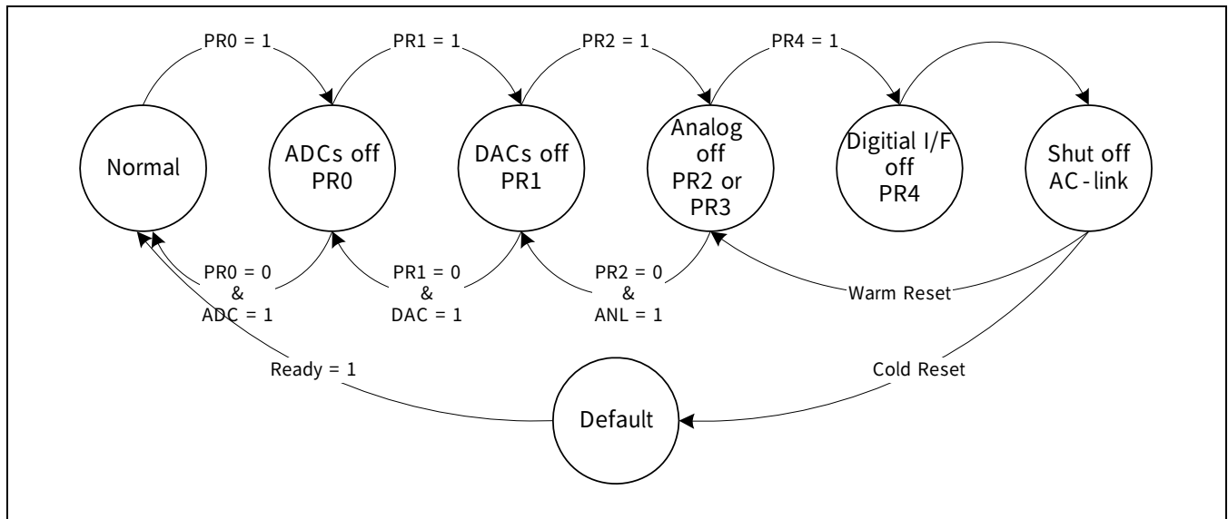
Figure 10.4-8 AC97 Power down/Power up Flow
