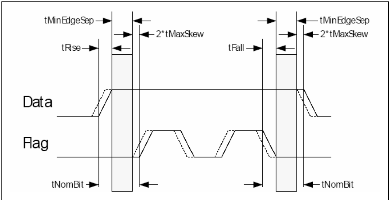
Figure 8.6-9 Waveform
