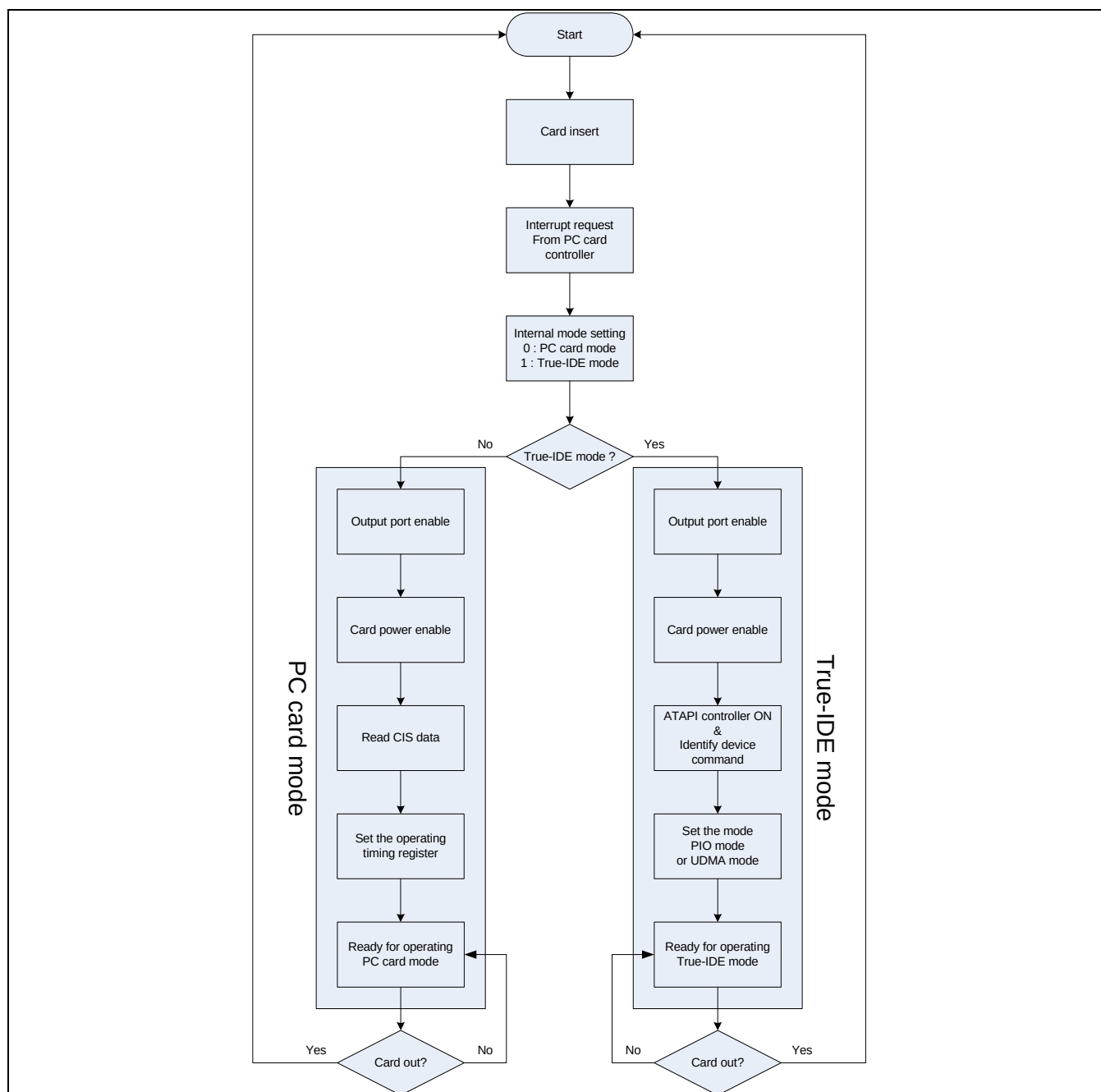
Figure 5.5-15 Basic Function Flow Chart
