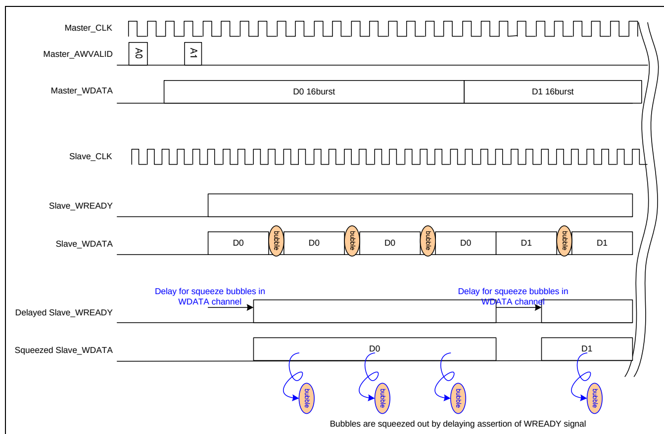
Figure 3.4-9 Write Data Bubble Squeezing Scheme in Async Bridge
