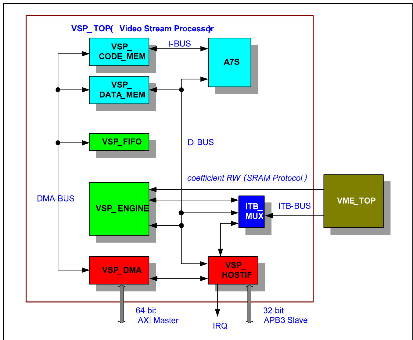
Figure 9.11-2 Video Stream Processor Block Diagram
