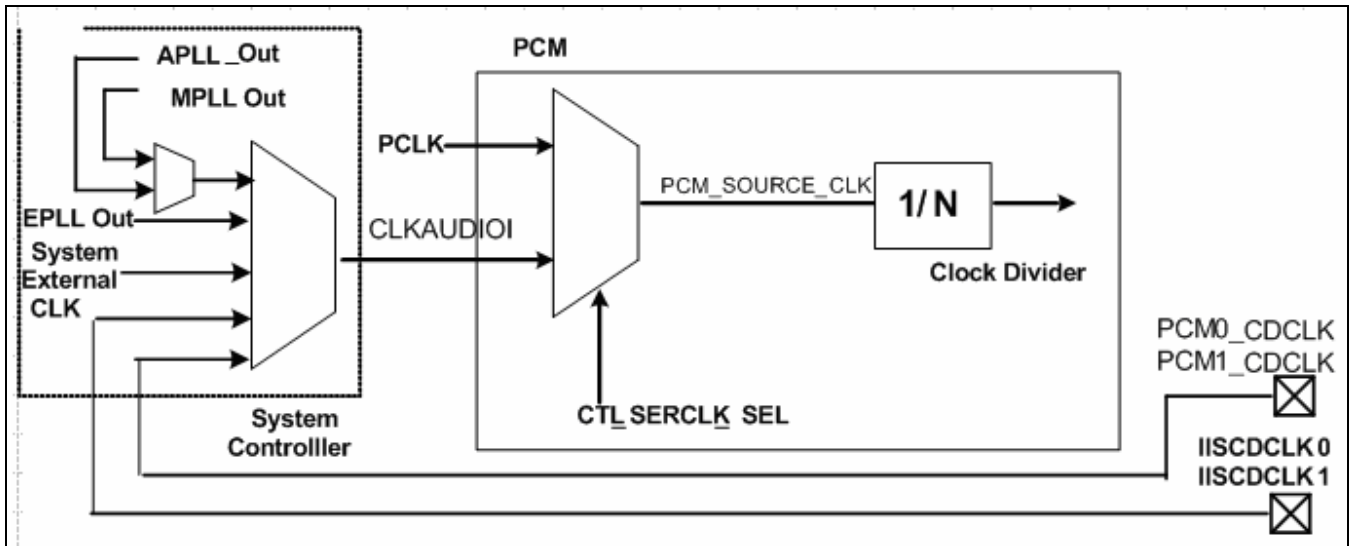
Figure 10.5-3 Input Clock Diagram for PCM
