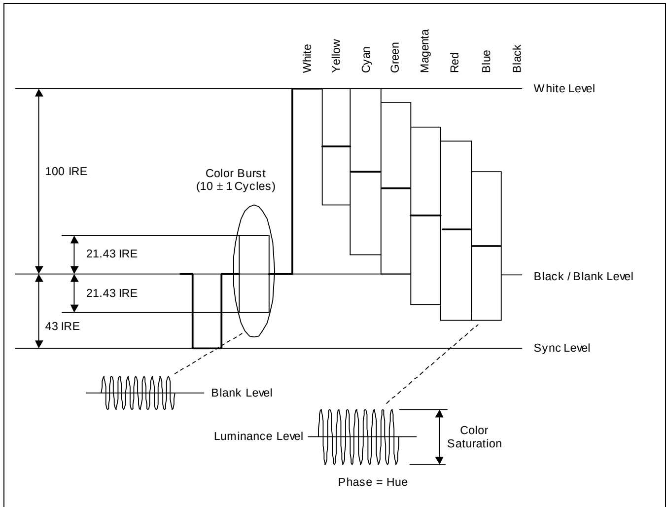
Figure 9.7-14 PAL (BGHDNc) Composite Video Signal with 75% Color Bars
