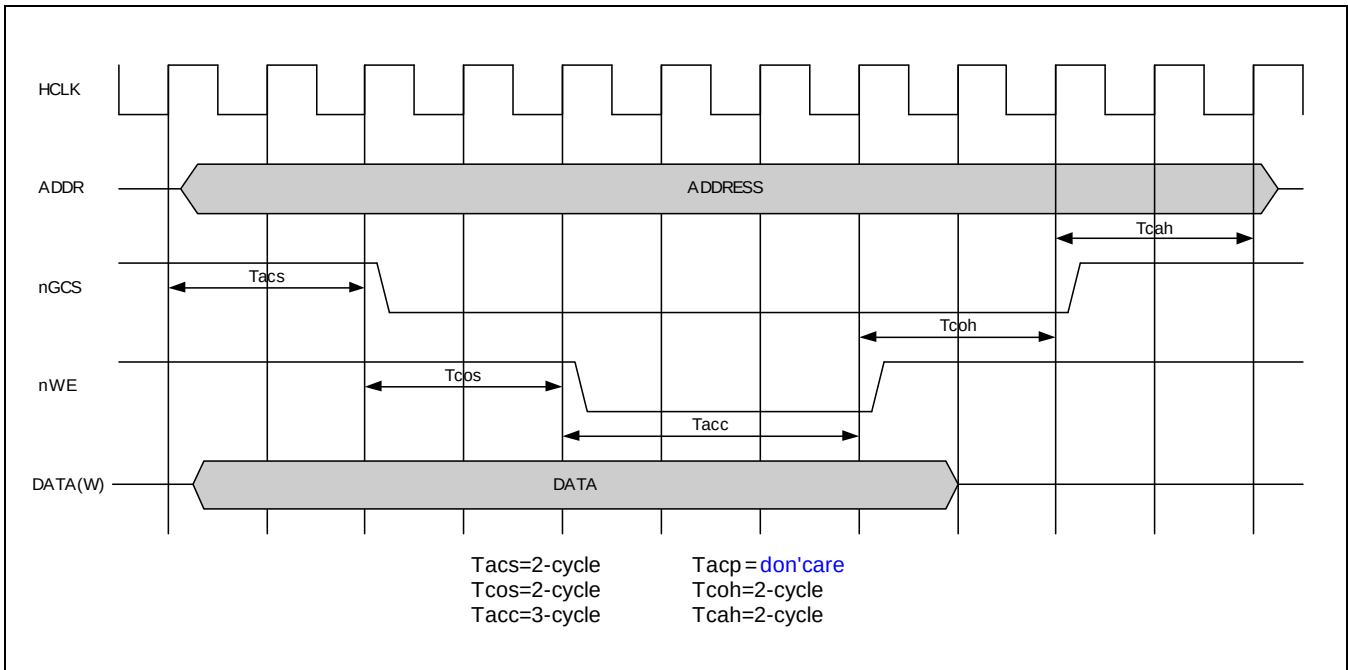
Figure 5.2-4 SMC Controller Write Timing Diagram
