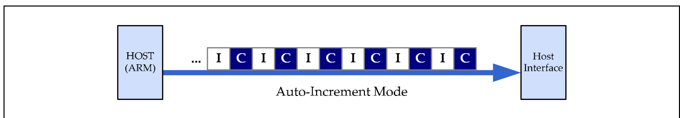
Figure 9.6- 6 Auto-Increment Mode
