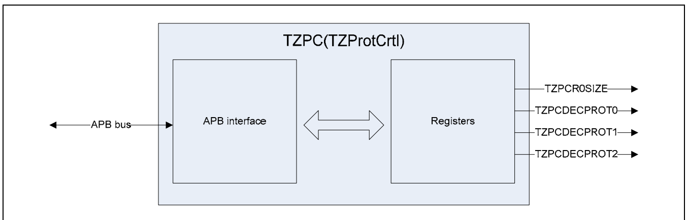
Figure 3.3-1 Block Diagram
