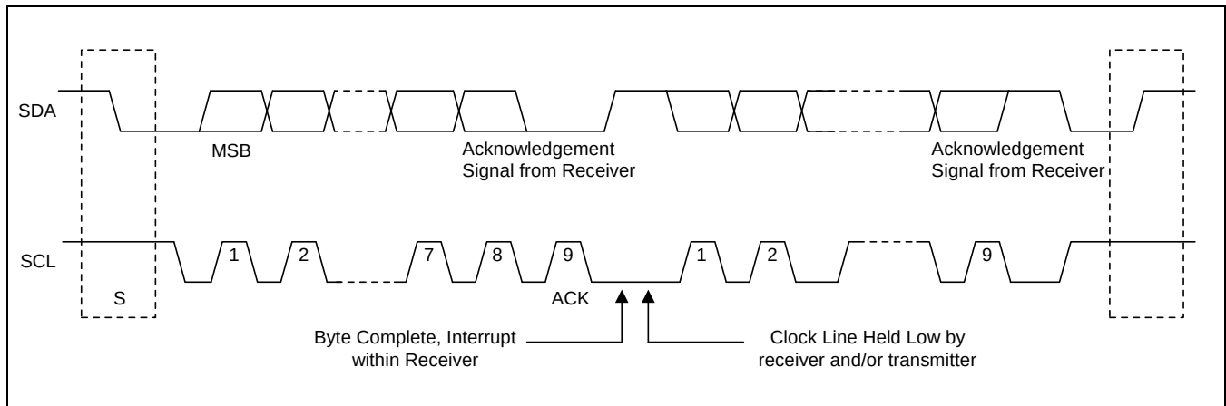
Figure 8.2-4 Data Transfer on the I 2 C-Bus
