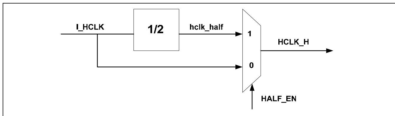
Figure 9.4-2 JPEG Half Clock
