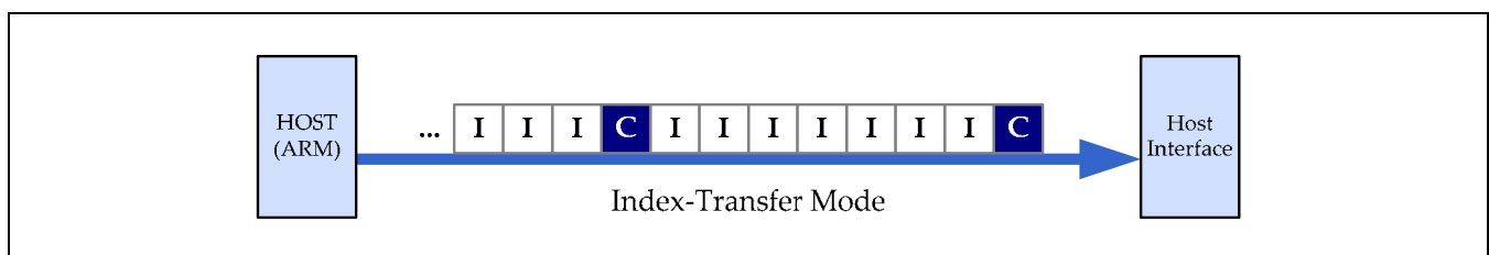
Figure 9.6- 8 Index-Transfer Mode
