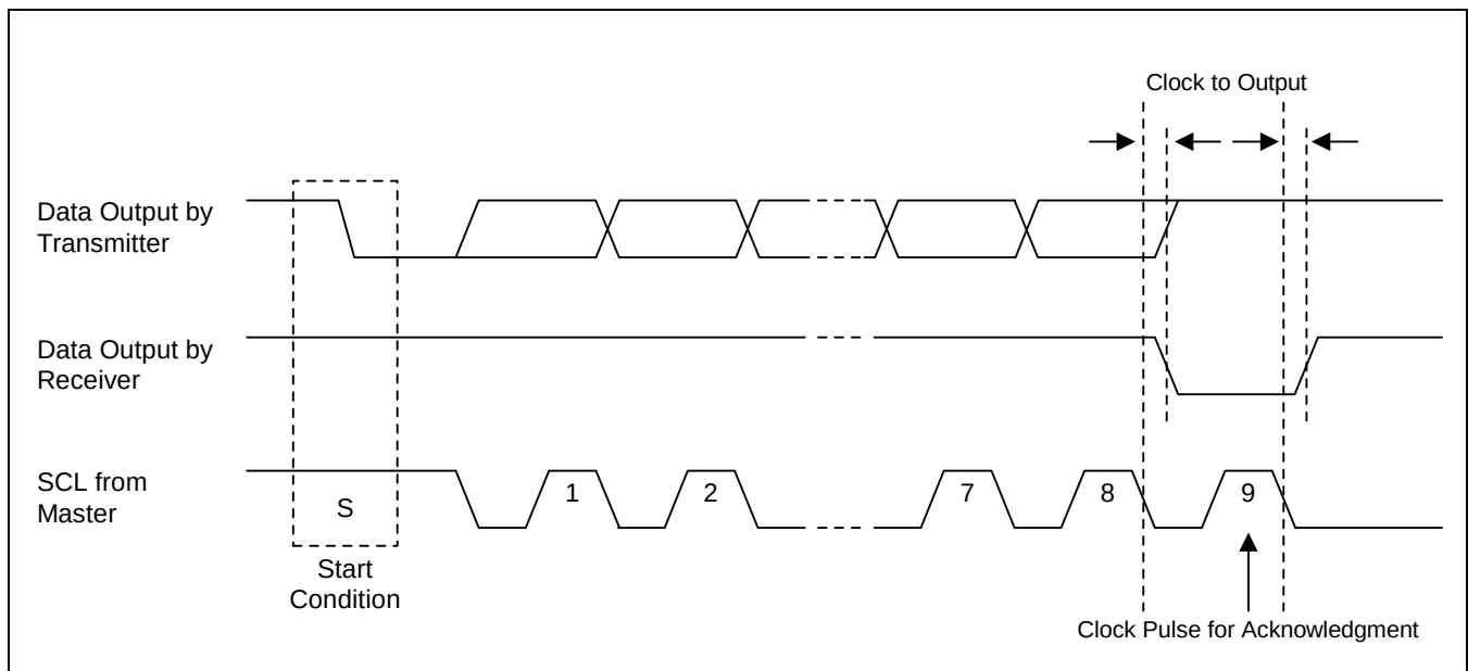
Figure 8.2-5 Acknowledge on the I 2 C-Bus
