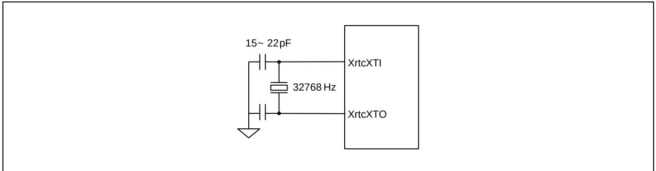
Figure 7.4-2 Main Oscillator Circuit Example
