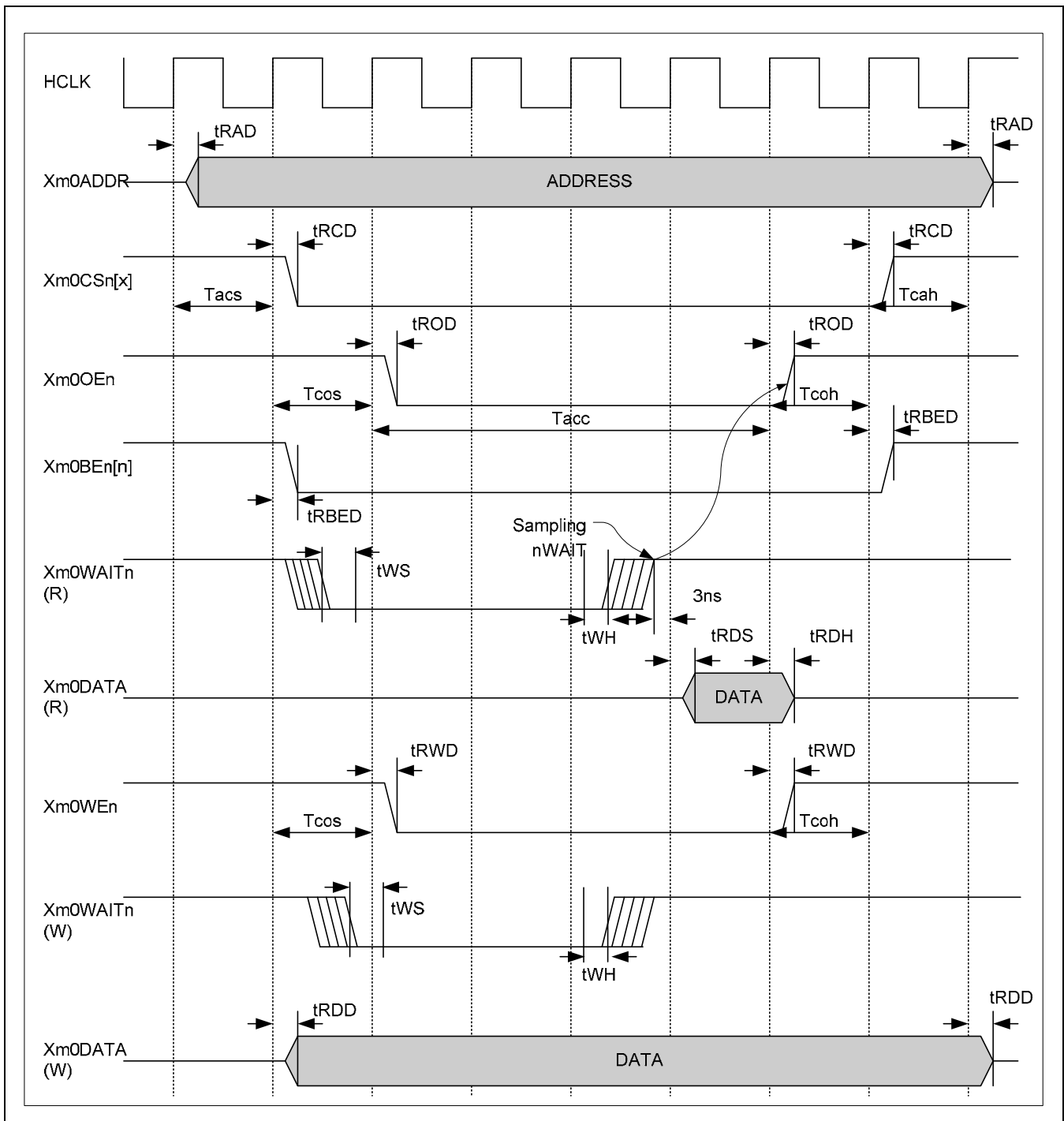
Figure 12.1- 6 ROM/ SRAM Timing ( T_{acs} = 0 , T_{cos} = 0 , T_{acc} = 2 , T_{coh} = 0 , T_{cah} = 0 , PMC = 0 , ST = 0 , DW = 16\text{-bit} )
