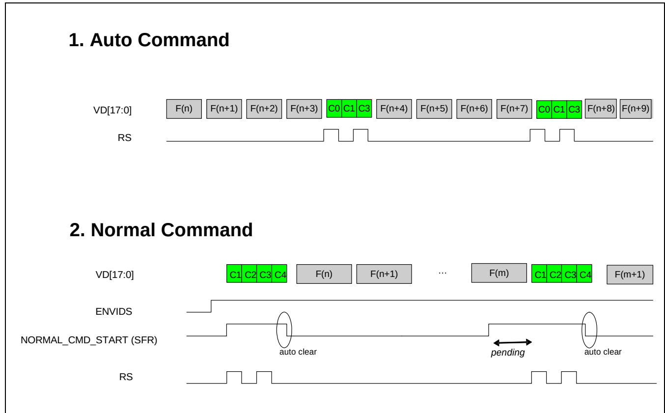
Figure 9.1- 9 Sending Command
