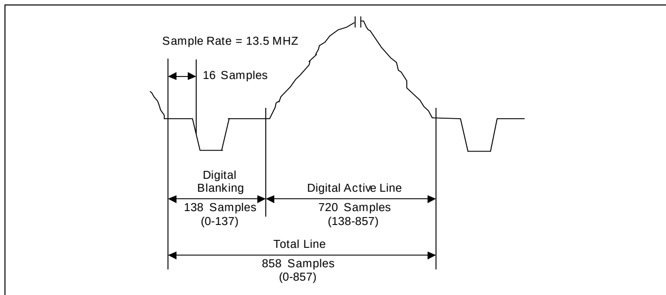
Figure 9.7-5 Horizontal Blanking and Active Video Timing @ 525/60 Hz
