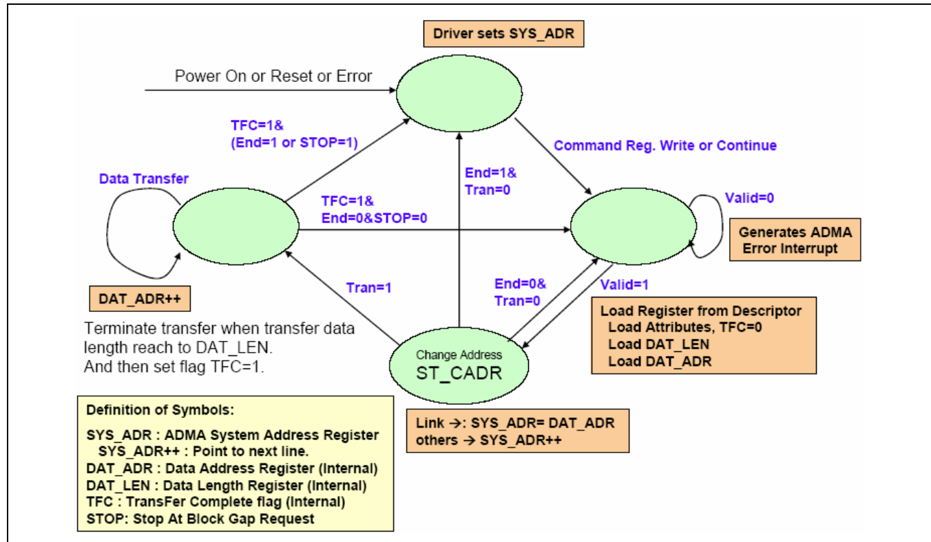
Figure 8.12- 16 State Diagram of the ADMA
