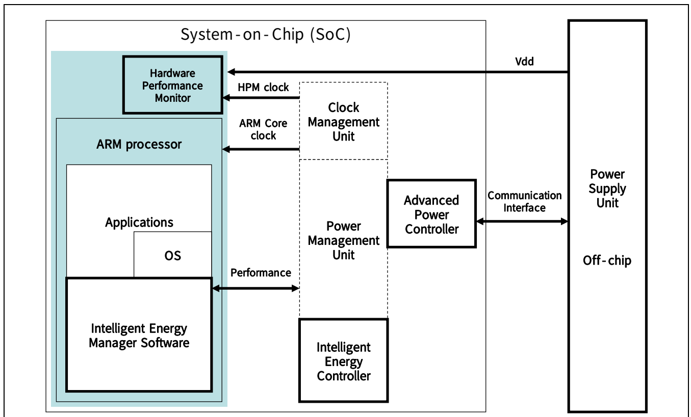
Figure 2.5-1 Intelligent Energy Manager Solution
