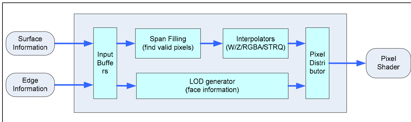
Figure 9.6- 16 Rasterizer Pipeline Overview
