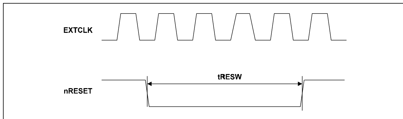
Figure 2.4- 6 Manual Reset Input Timing
