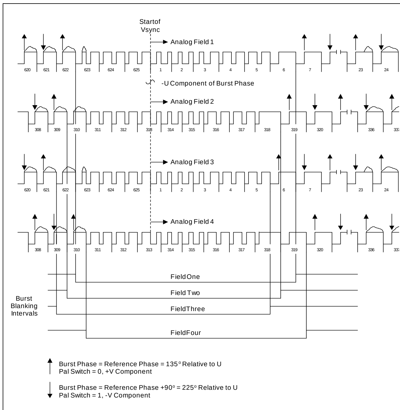
Figure 9.7-3 Field PAL (BGHIDNc) Sequence and Burst Blanking
