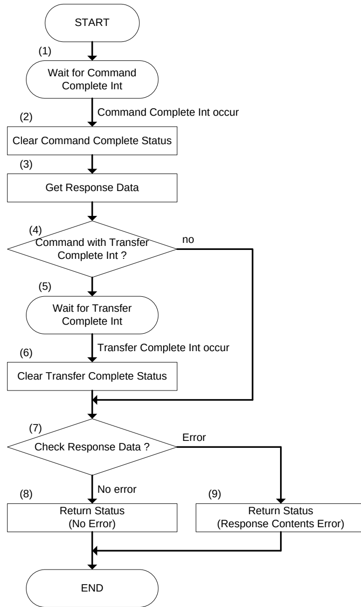
Figure 8.12-10 Command Complete Sequence
