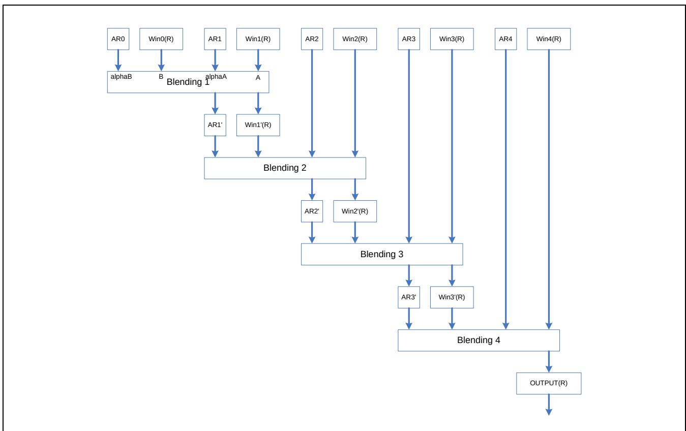
Figure9.1-6 Blending Diagram
