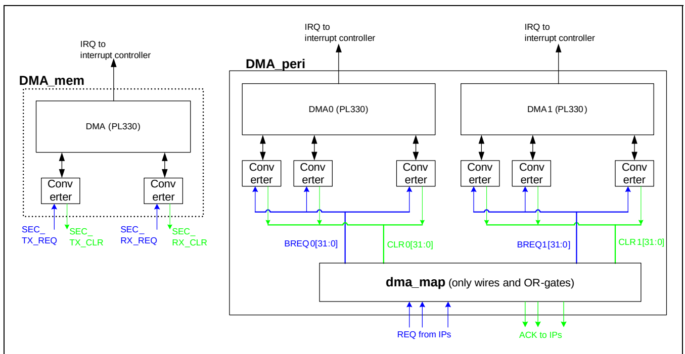
Figure 6.1-1 Two DMA Tops
