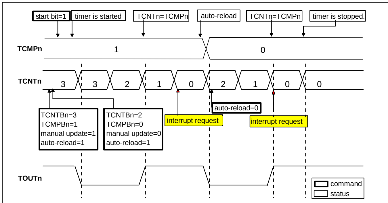
Figure 7.1-3 Timer Operations
