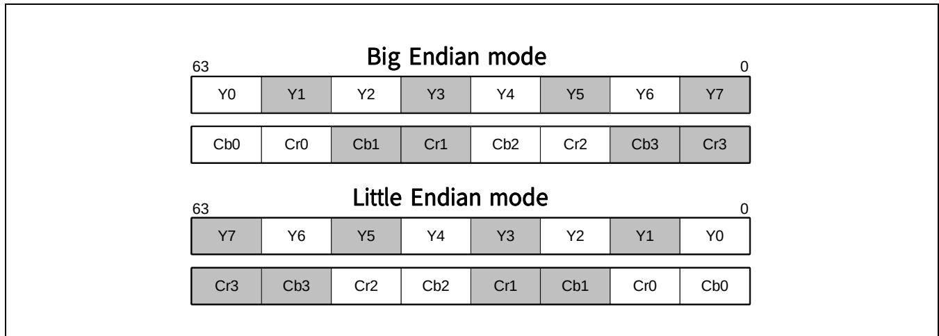
Figure 9.8-6 Endian Mode
