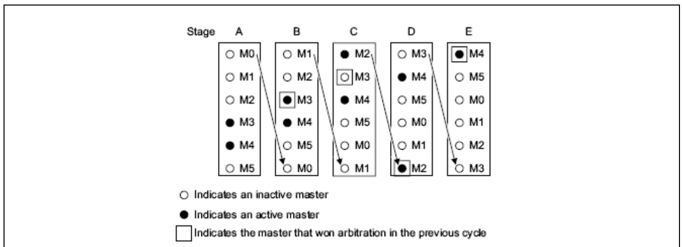
Figure 3.1-3 Example Operation of RR Arbitration Scheme
