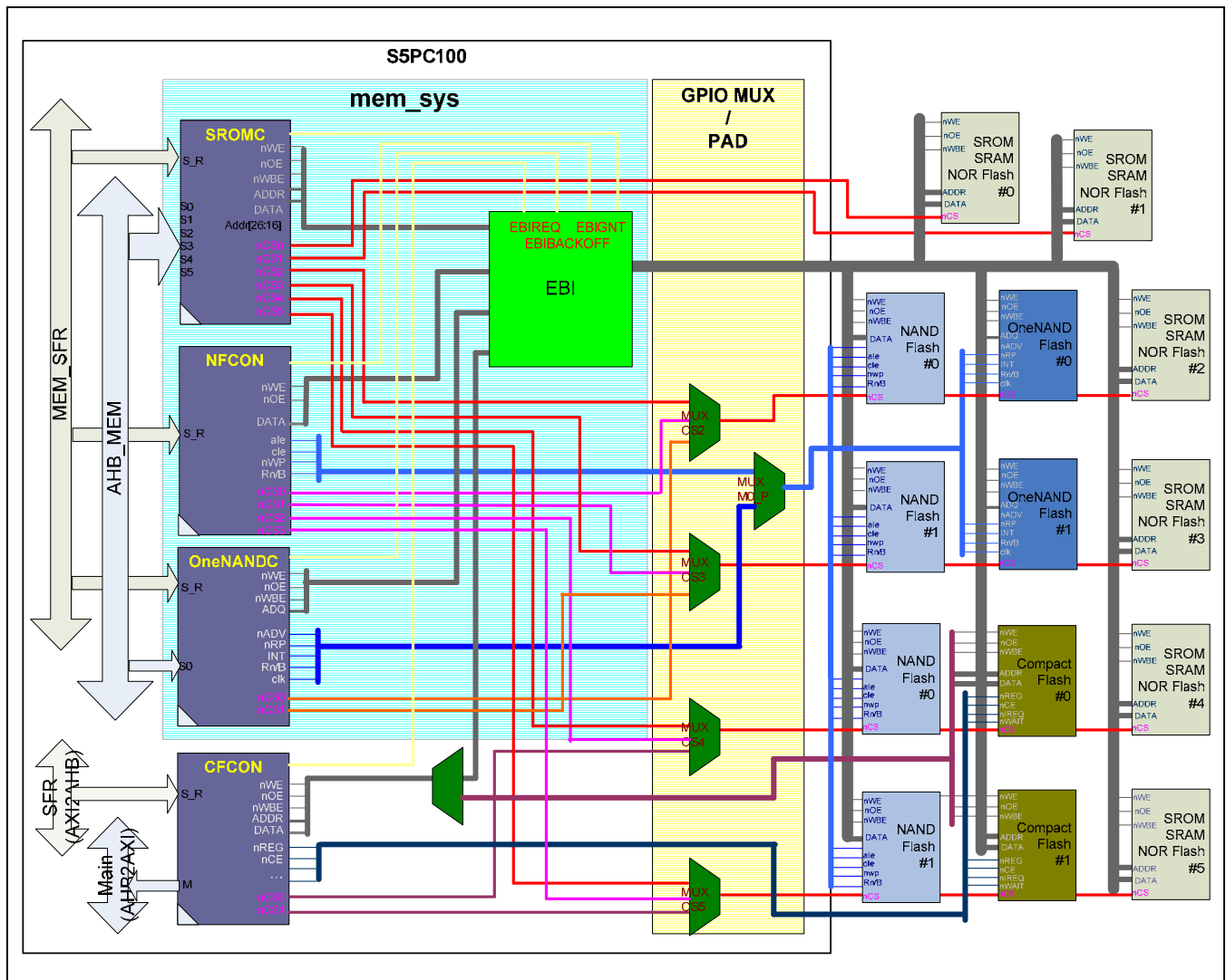
Figure 5.6-1 Memory Interface Through EBI
