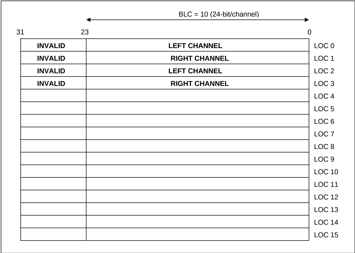
Figure 10.3-7 RX FIFO Structure for BLC = 10 (24-bit/channel)
