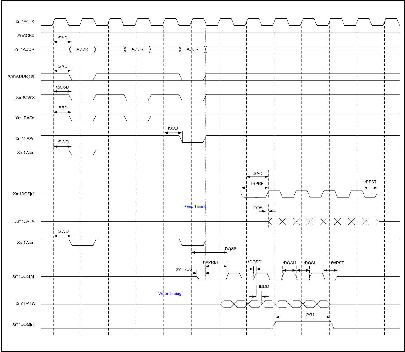
Figure 12.1- 9 LPDDR1 SDRAM Read / Write Timing (Trp = 2, Trcd = 2, Tcl = 2, DW = 16-bit)
