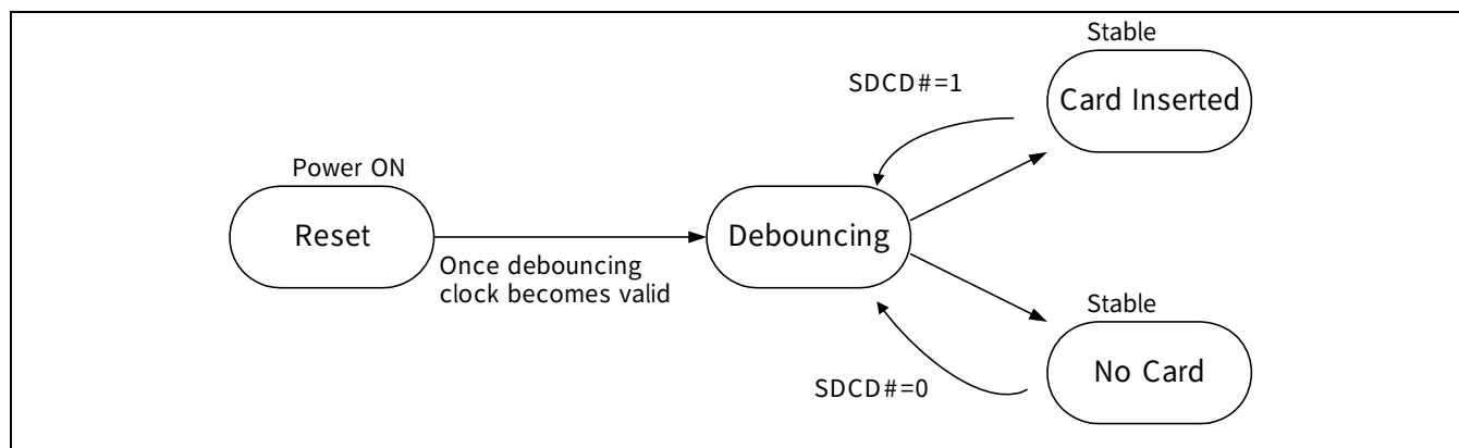
Figure 8.12-17 Card Detect State
