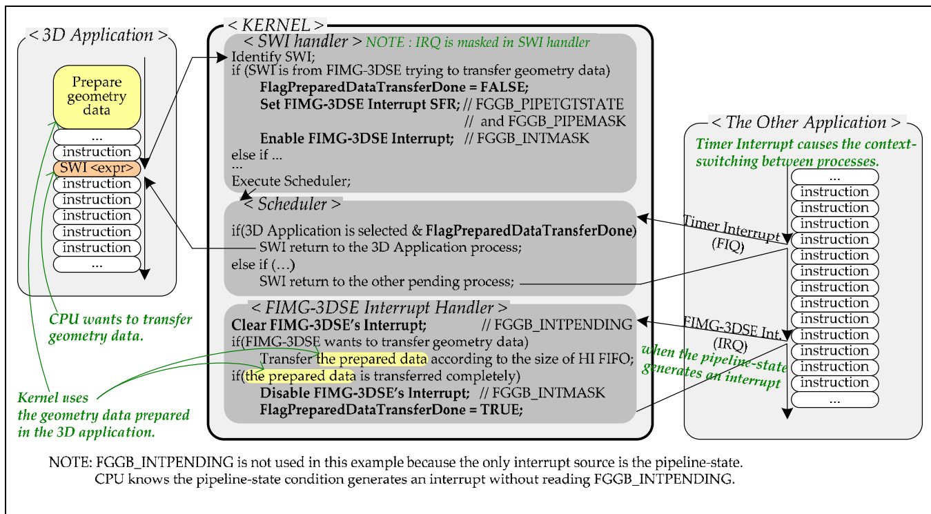
Figure 9.6- 3 A Simple Example of Transferring Geometry Data. (Other Methods Can be Used as Well.)
