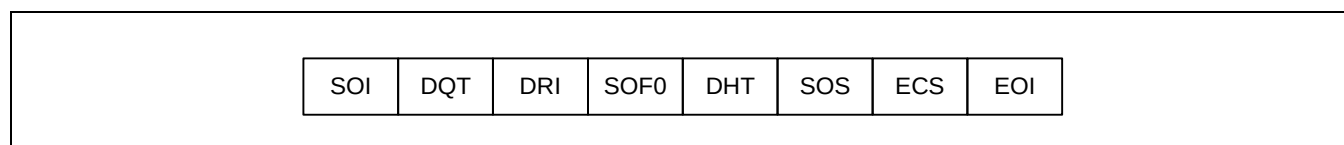
Figure 9.4- 7 Bitstream of Compressed File
