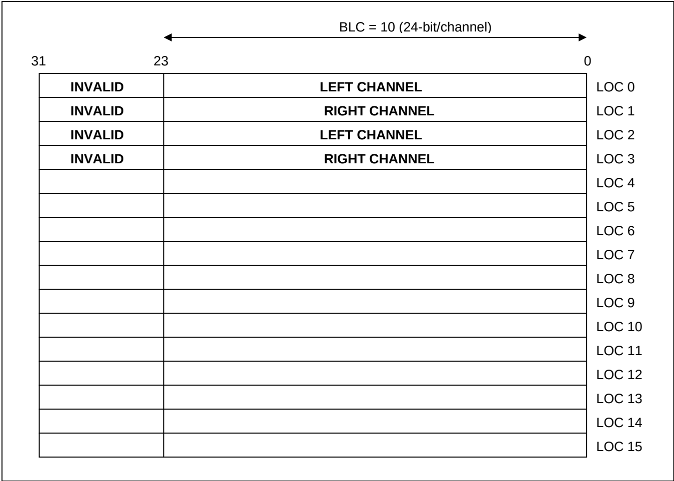
Figure 10.2-7 TX FIFO Structure for BLC = 10 (24-bit/channel)
