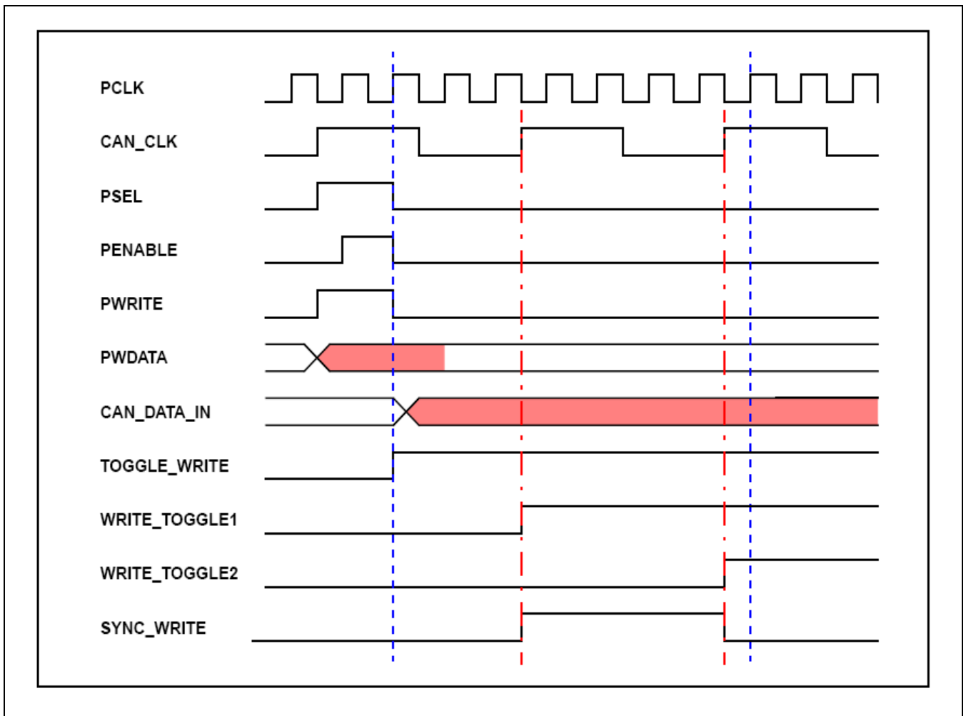
Figure 8.5-6 APB2 Write Timing
