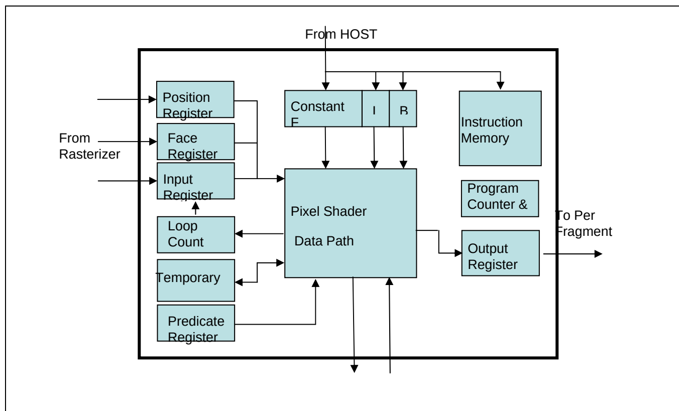
Figure 9.6- 17 Pixel Shader Block Diagram
