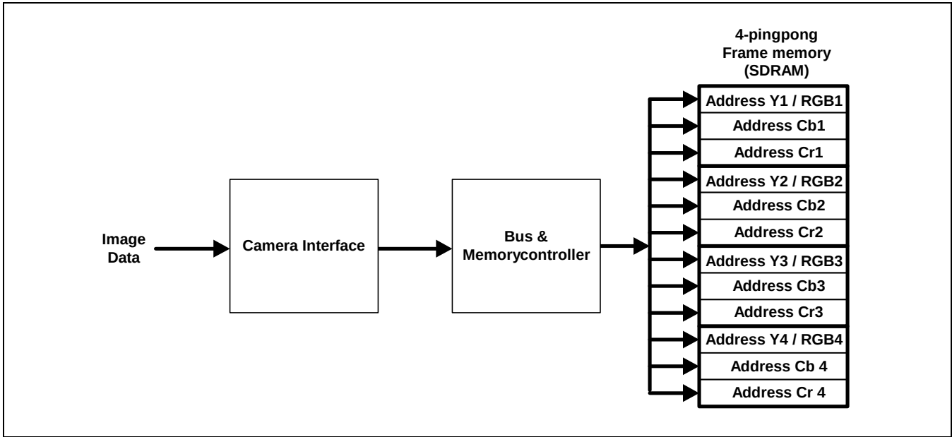
Figure 9.3-10 Ping-pong Memory Hierarchy
