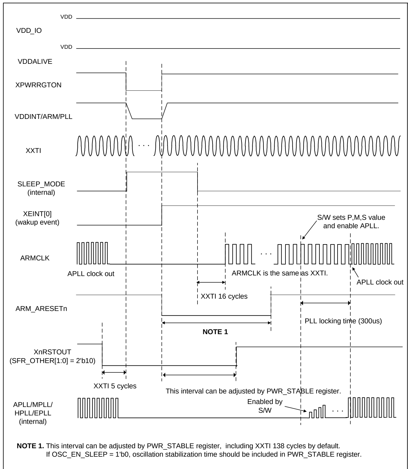
Figure 2.4-15 SLEEP Mode Wakeup Timing
