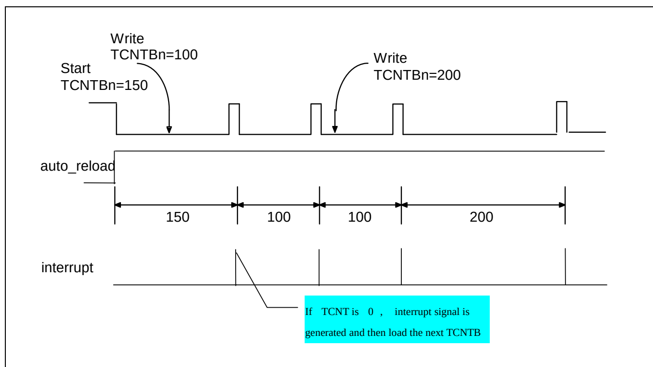
Figure 7.1-4 Example of Double Buffering Feature
