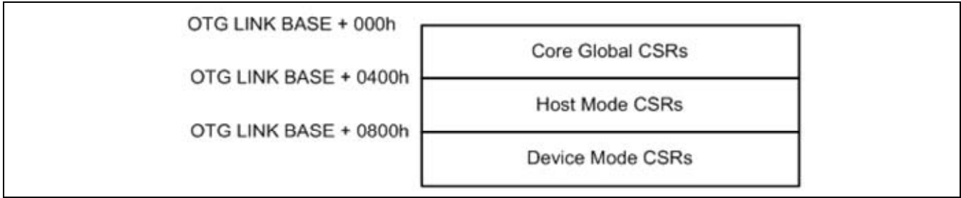
Figure 8.10-2 OTG Link CSR Memory Map
