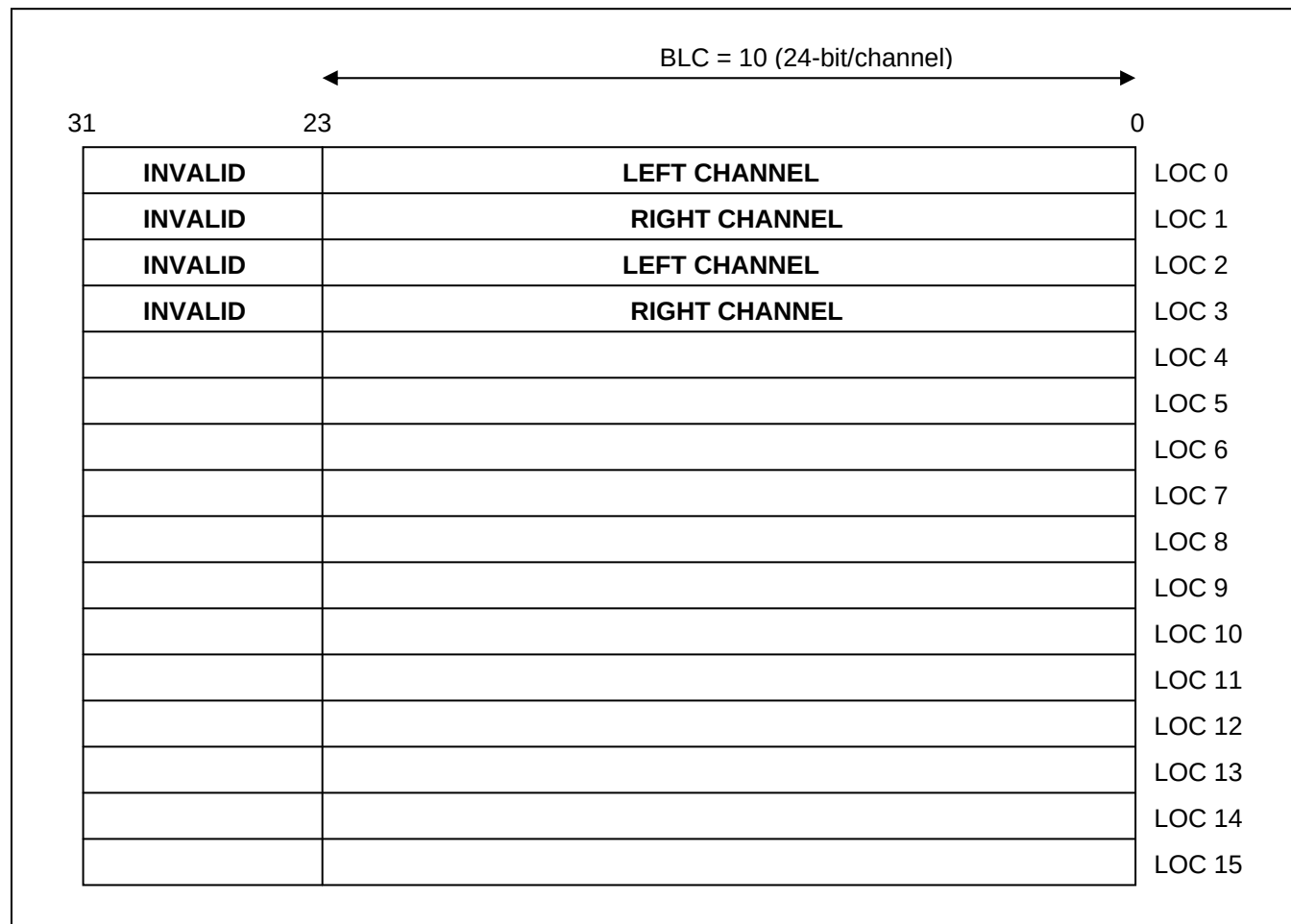
Figure 10.2-9 RX FIFO Structure for BLC = 10 (24-bit/channel)
