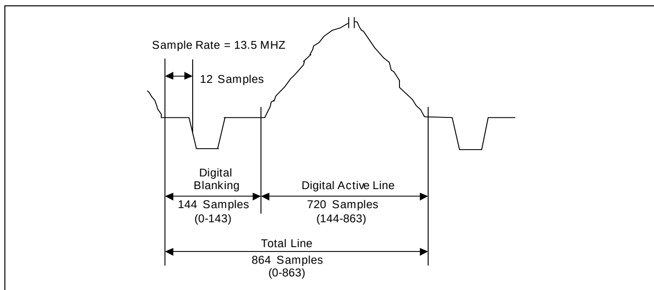
Figure 9.7-6 Horizontal Blanking and Active Video Timing @ 625/50 Hz
