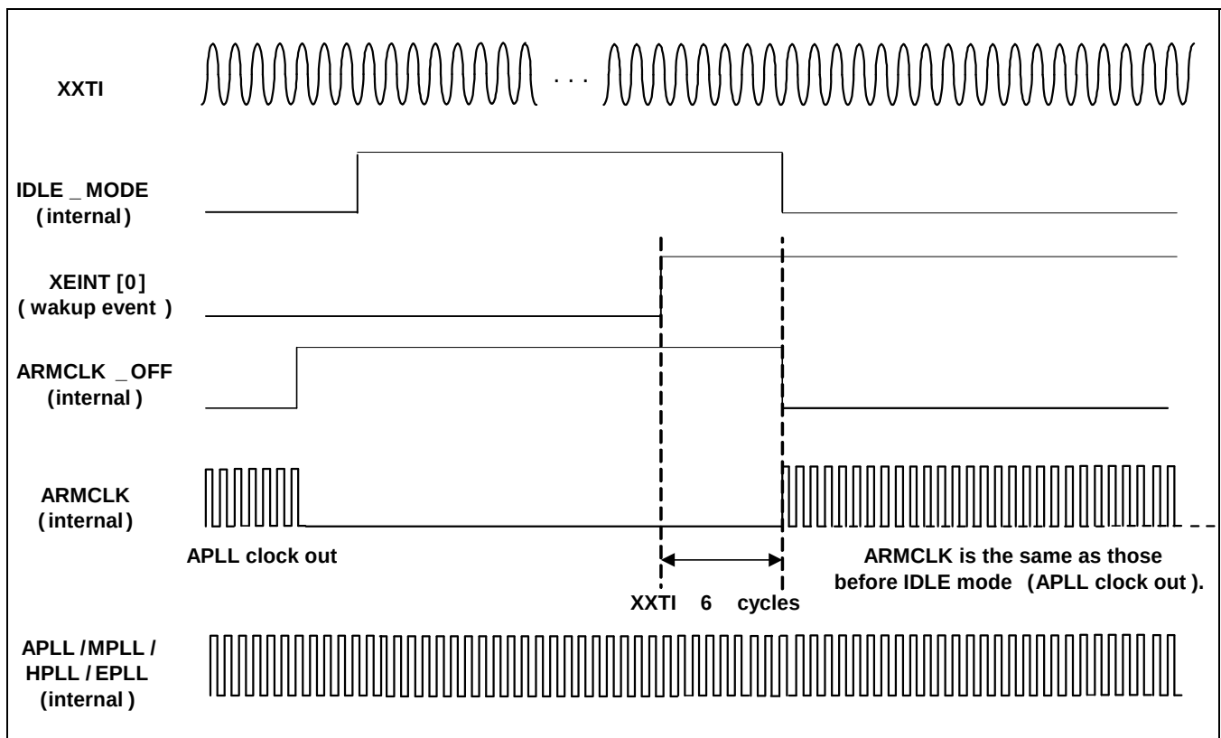
Figure 2.4-9 IDLE Mode Wakeup Timing
