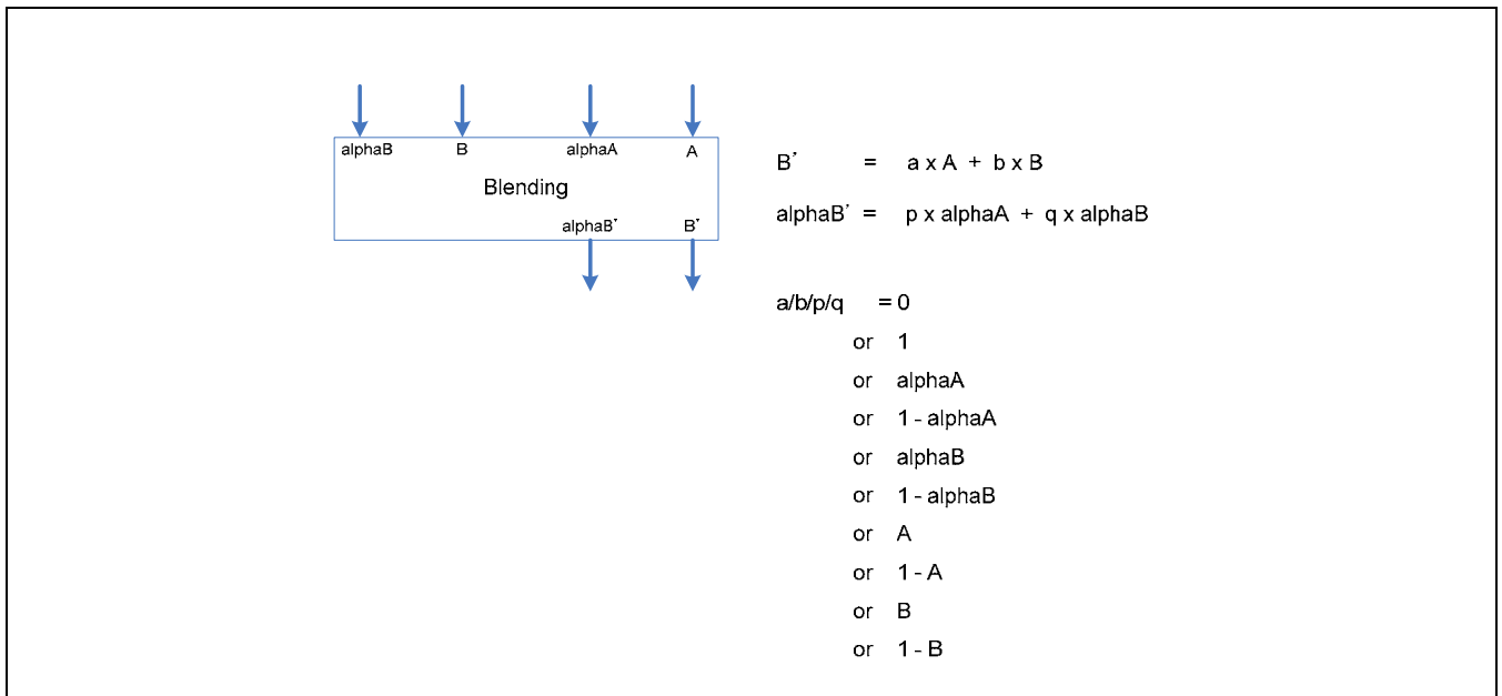
Figure 9.1-5 Blending Equation
