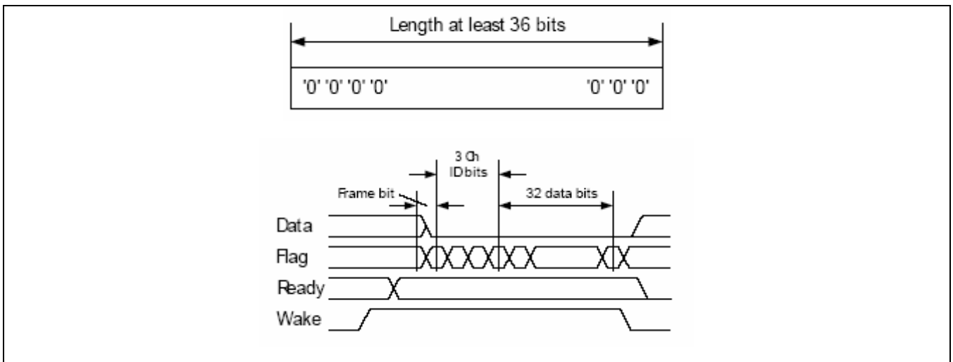
Figure 8.6-13 Break Frame
