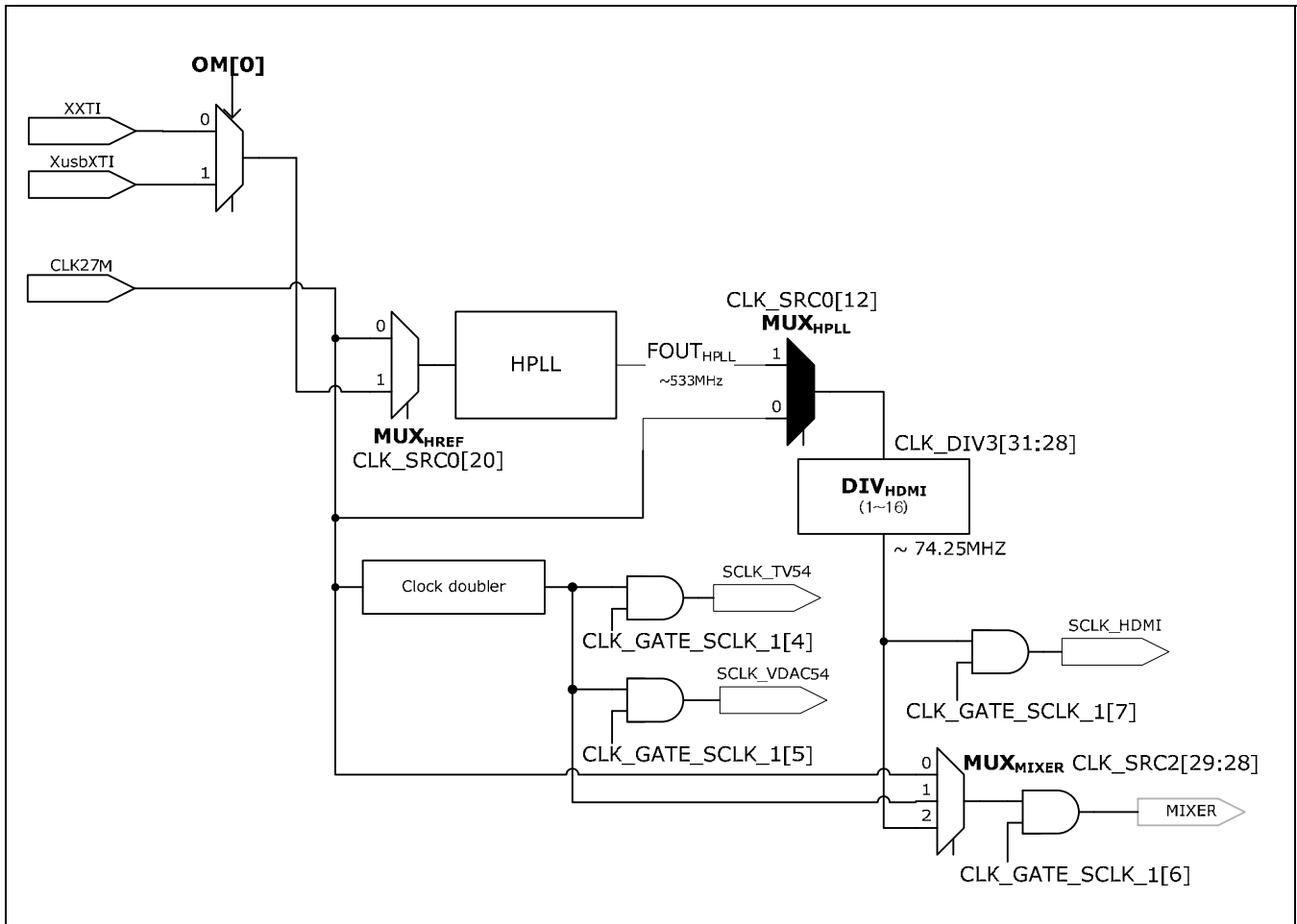
Figure 2.3-8 TV Clock
