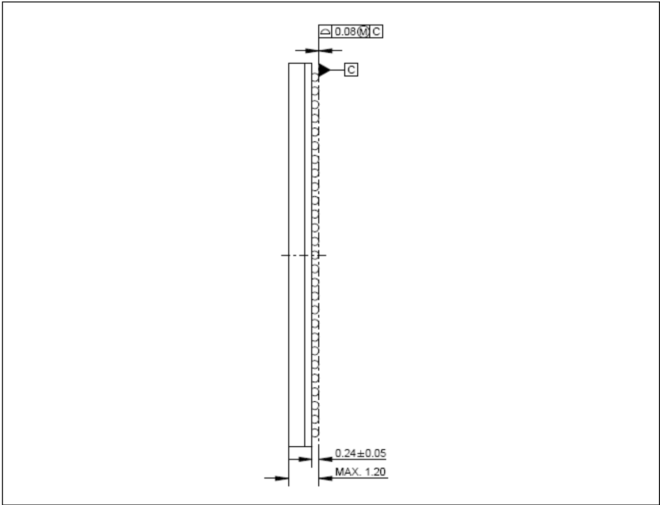
Figure 1.3- 2 S5PC100 Package Dimension (521-FCFBGA) – Side View
