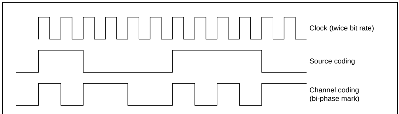
Figure 10.6-4 Channel Coding
