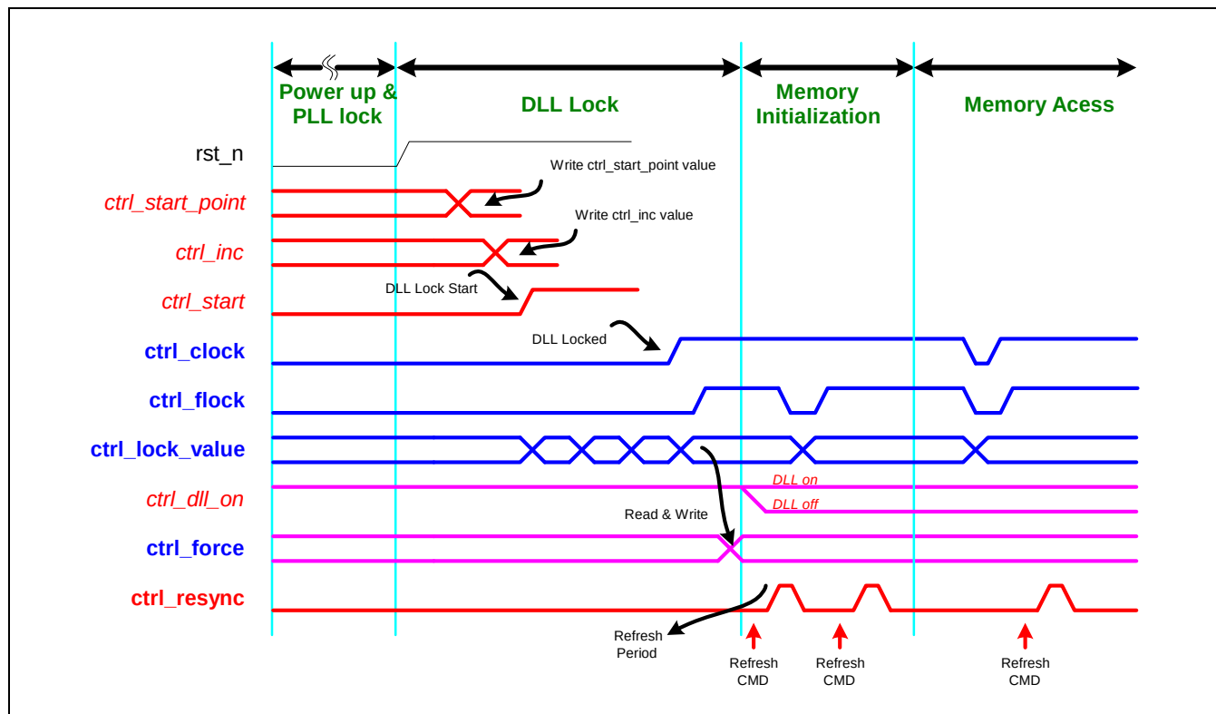
Figure 5.1-10 DLL Lock Procedure
