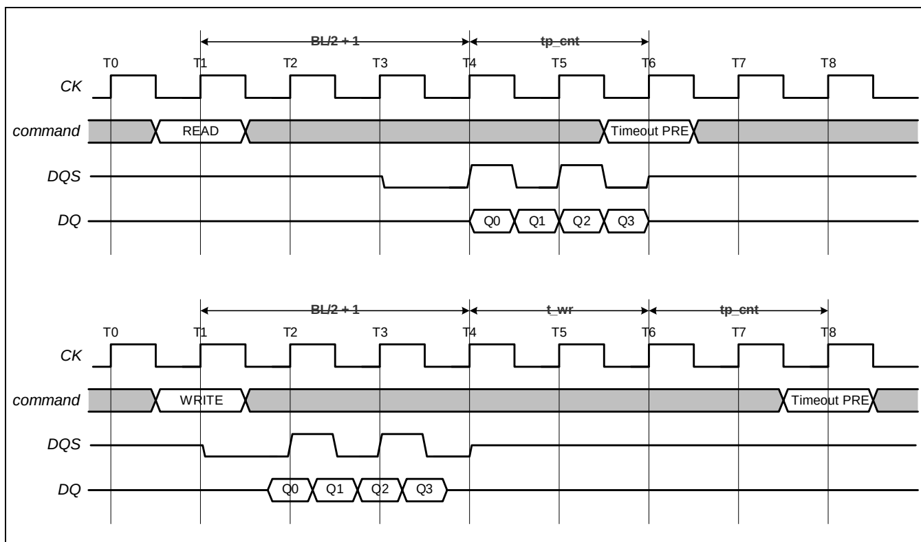
Figure 5.1-4 Timing Diagram of Timeout Precharge
