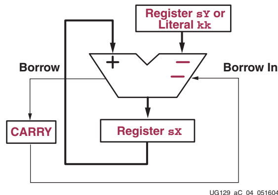
Figure C-10: SUBCY Instruction
