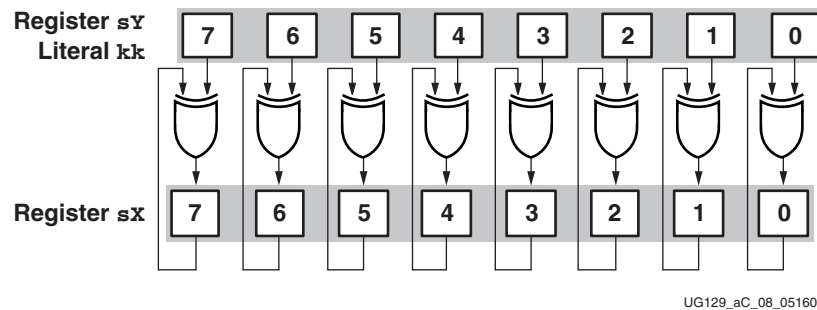
Figure C-13: XOR Operation
